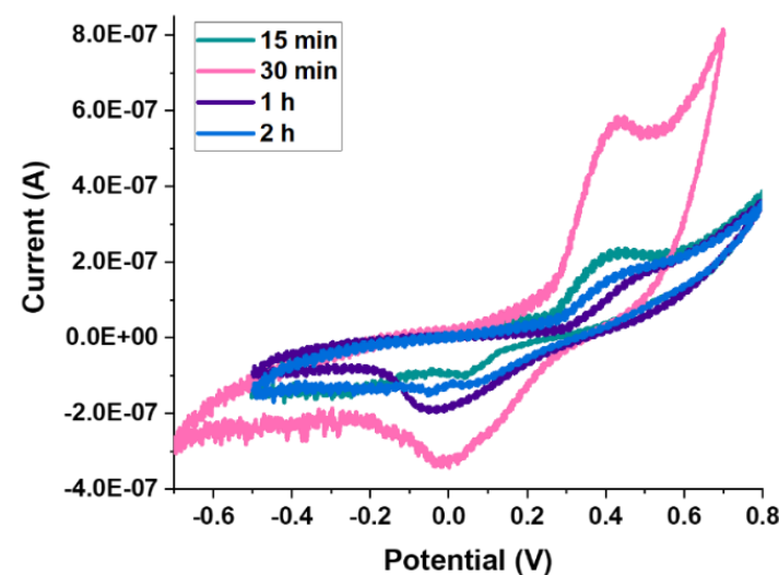
Figure 2. Effect of the cure time on the electrochemical performance of the sensors. CV analysis performed on membranes doped with 2% of glycerine and screen-printed with a Chi-LaA-AgNW dispersion, where the Chi:AgNW mass ratio is 1:1. Ink layers cured for 15 min, 30 min, 1 h or 2 h, at 75 °C.
