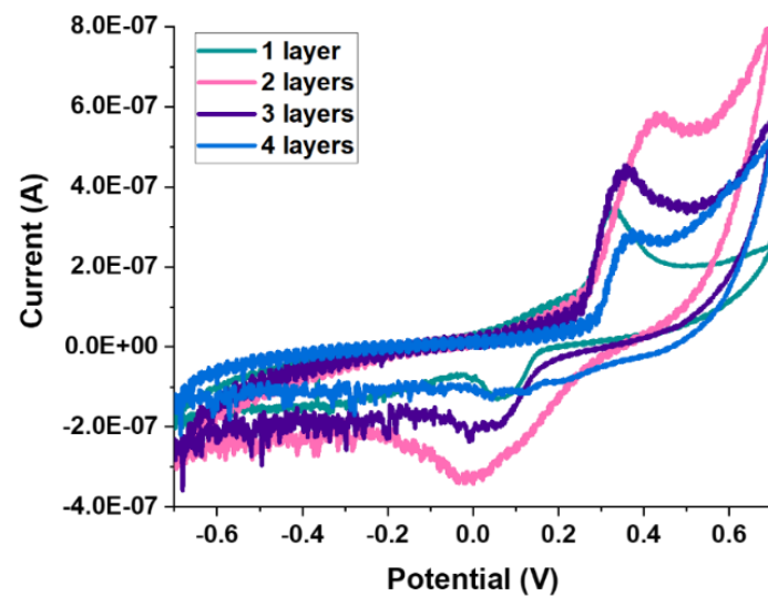
Figure 1. Effect of the number of ink layers on the electrochemical performance of the sensors. CV analysis performed on membranes doped with 2% of glycerine and screen-printed with 1 to 4 layers of a Chi-LaA-AgNW dispersion, where the Chi:AgNW mass ratio is 1:1. Ink layers cured for 30 min, at 75 °C.
