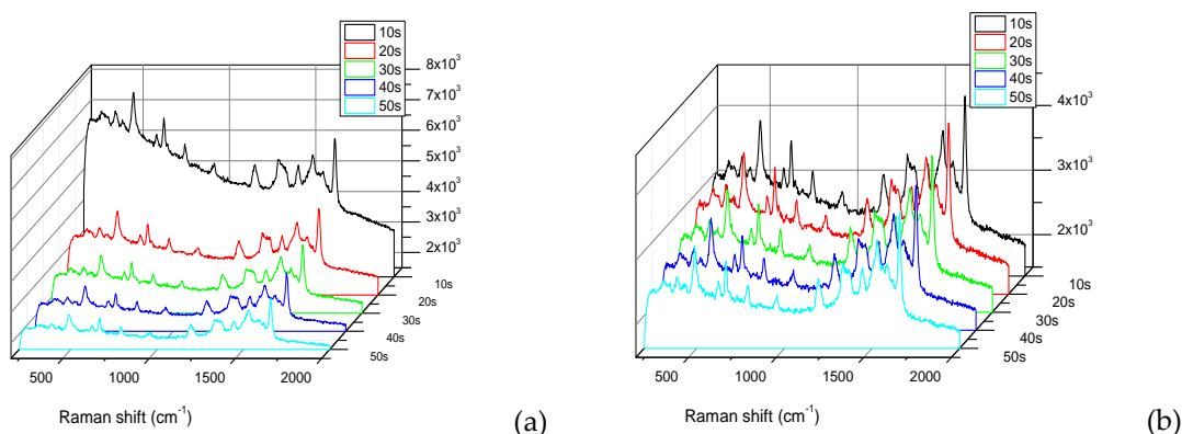
Figure 3. Dependence of the intensity of Raman scattering and background fluorescence of fluorescein on the time under irradiation of 3D Au NP nanostructures with different film thickness d , the average diameter D of Au nanoparticles, and the number N of Au grains per 0.0625 \mu\text{m}^2 : (a) d=24 \text{ nm} , D=19 \text{ nm} , N=358 ; (b) d=19.5 \text{ nm} , D=16.5 , N=167 .
