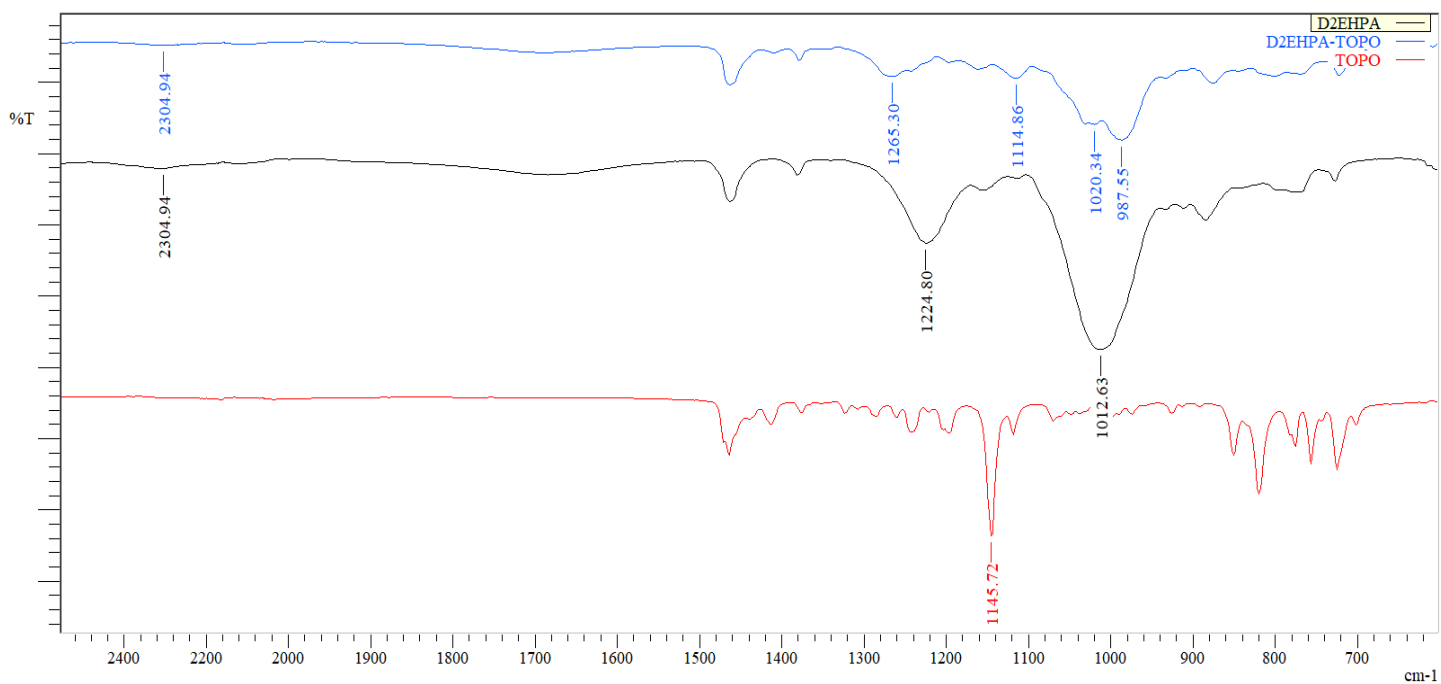
Figure S1. Infrared spectra of D2EHPA, HDES and TOPO.
