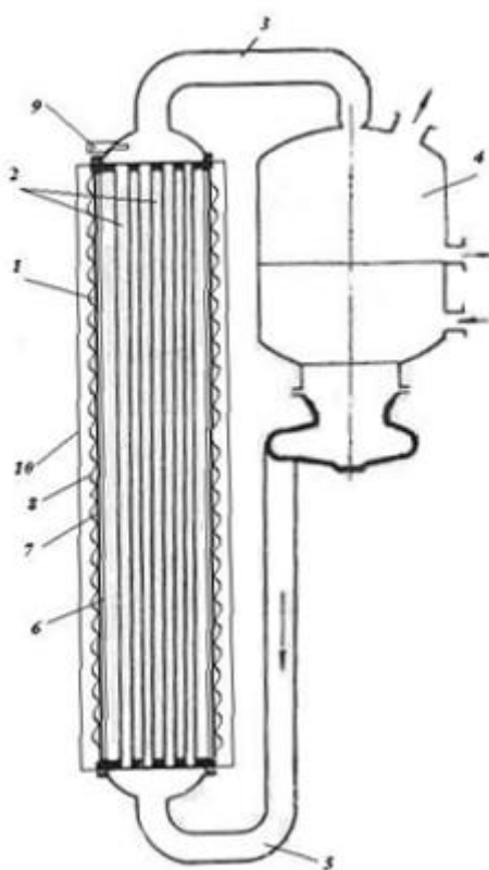
Figure 1. Induction evaporator.
