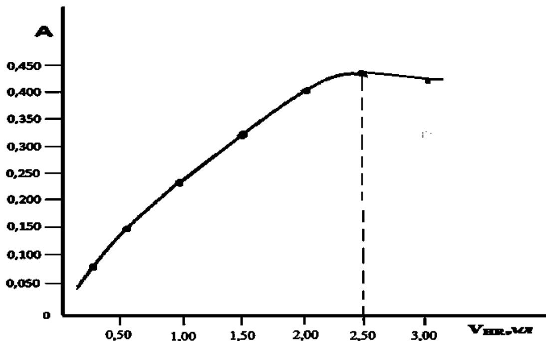
Figure 3. Graph of dependence of the optical density of the complex compound (FeR) on the amount of added reagent.
