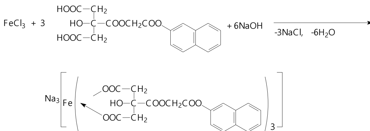
Figure 8. Fe:HR=1:3 ratio complex formation reaction equation.
