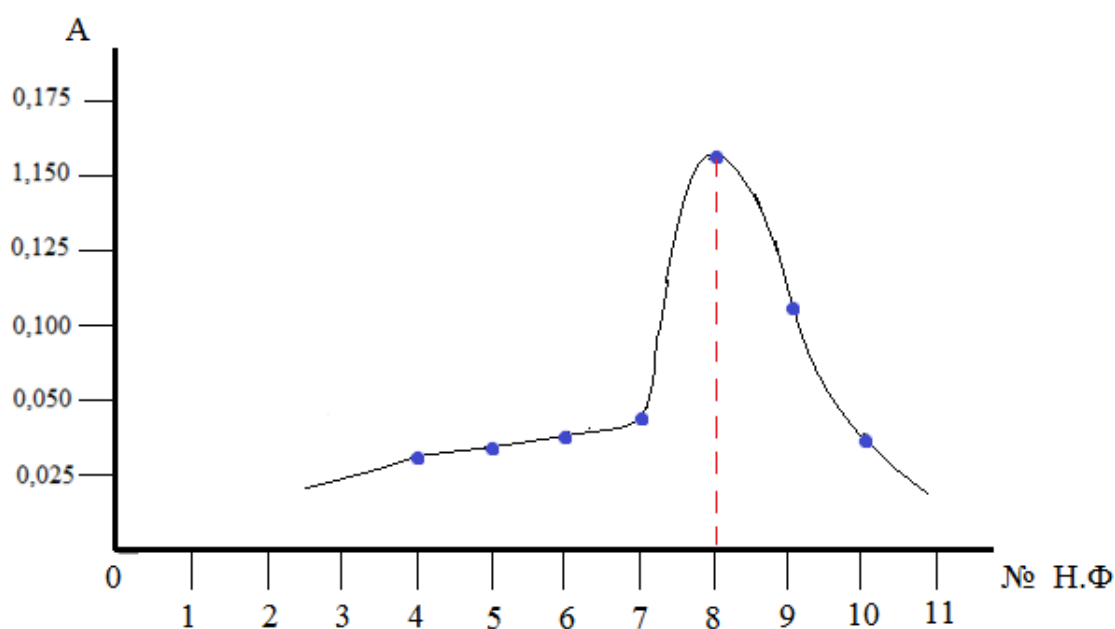
Figure 2. Dependence of the optical density of the FeR complex on the light filter .
