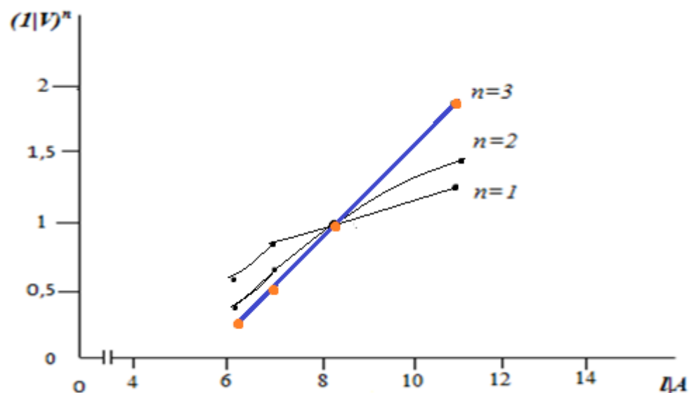
Figure 7. Graph of determination of the composition of the complex of iron (III) with 2-naphthylcarboxymethylene citrate using Asmus' straight line method.
