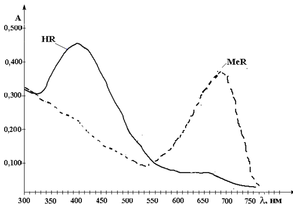
Figure 5. Absorption spectrum of iron(III) complex with 2-naphthylcarboxymethylene citrate reagent.
