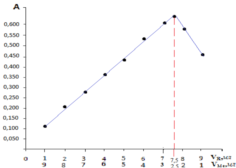
Figure 6. The curve for determining the composition of the complex compound (FeR) using the isomolar series method.
