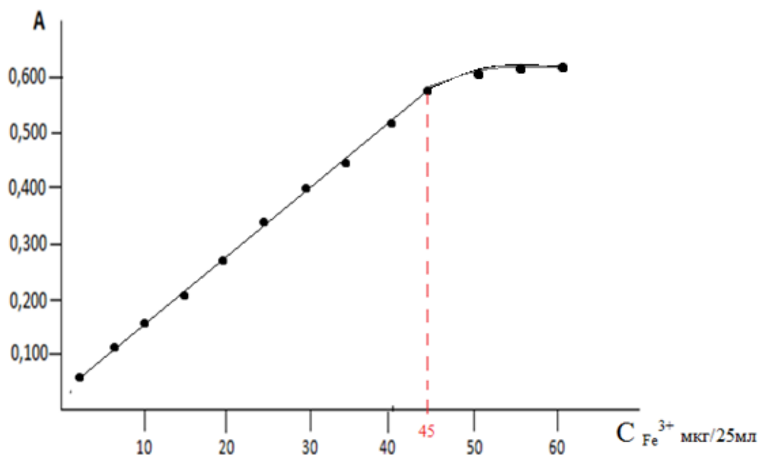
Figure 4. The graph of optical density depending on the amount of added Iron(III).
