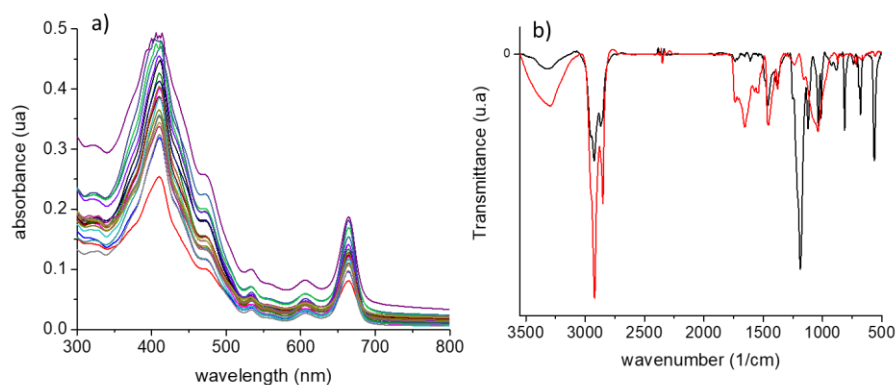
Figure 1. a) UV-Vis spectra of the extracts obtained from manure. b) FTIR spectra for a representative sample of feces in the presence of commercial archaeol (black) and in the absence of commercial archaeol (red).
