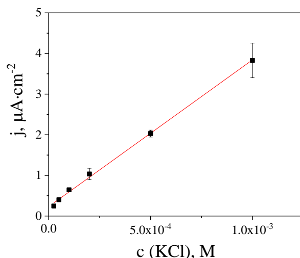
Figure 3. Calibration plot in flow-injection amperometric mode for PB nanoparticles modified electrode covered with K + -selective membrane (E=-0.1 V; 50 mM Bis-Tris, pH 6.0).
