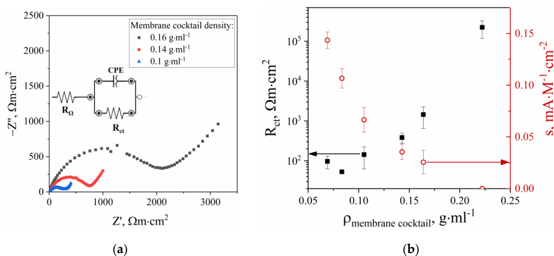
Figure 2. (a) Nyquist plots from EIS of sensors based on PB nanoparticles coated on ISM with various composition. Inset: the equivalent circuit used in the fitting. ( E_{dc}=0.1 V; 0.1 M KCl/HCl). (b) Dependence of the charge transfer resistance (■) and the sensitivity of the sensors (●) on the ion-selective membrane cocktail density.
