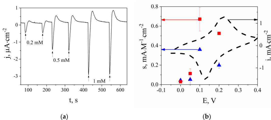
Figure 1. (a) Flow-injection amperometry of KCl solutions in 0.1 M HCl using PB nanoparticles- modified screen-printed electrodes without ion-selective membrane, E_{dc} = 0.1 V. (b) The dependence of the sensitivity of PB nanoparticles modified electrodes on the potential in the amperometric determination of potassium (■) and sodium (▲) ions (0.1 M HCl); corresponding sensor cyclic voltammogram (0.1 M KCl/HCl; 40 mV/s).
