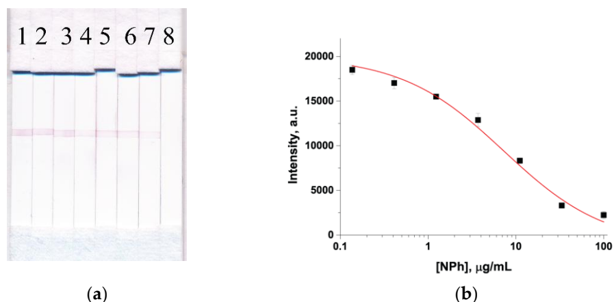
Figure 4. Inverted scheme of ICA: (a) Scanned image of test strips after application standard solutions of NPh of the following concentrations (1-8): 0; 0.1; 0.4; 1.2; 3.7; 11; 33; 100 \mu\text{g/mL} (a); calibration curve of NPs detection (n=3) (b).
