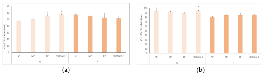
Figure 1. (a) Antioxidant capacity (Q-ABTS) and (b) hydroxyl radical scavenger (Q-HRS) activity of gastrointestinal (GI) and colonic fermentation (F) fractions of melanoidins. Asterisk (*) indicates significant differences between the values.
