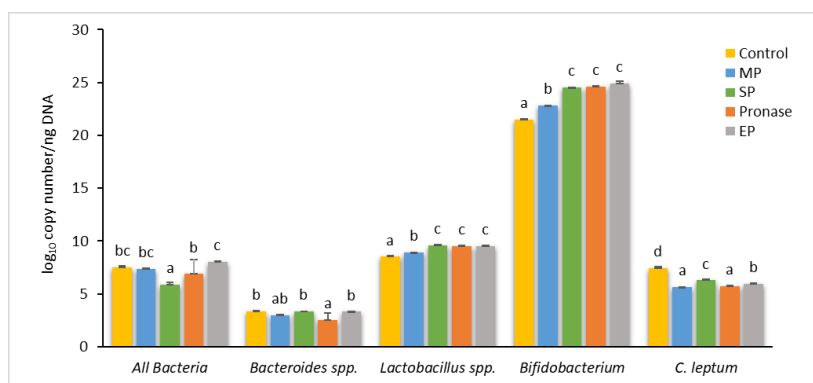
Figure 2. Microbiota composition in caecal samples treated with melanoidins. The results are shown as mean ± standard deviation (n = 3), the statistic was represented by performing a simple ANOVA in each bacterial strain comparing the control without melanoidins with bioaccessible samples.
