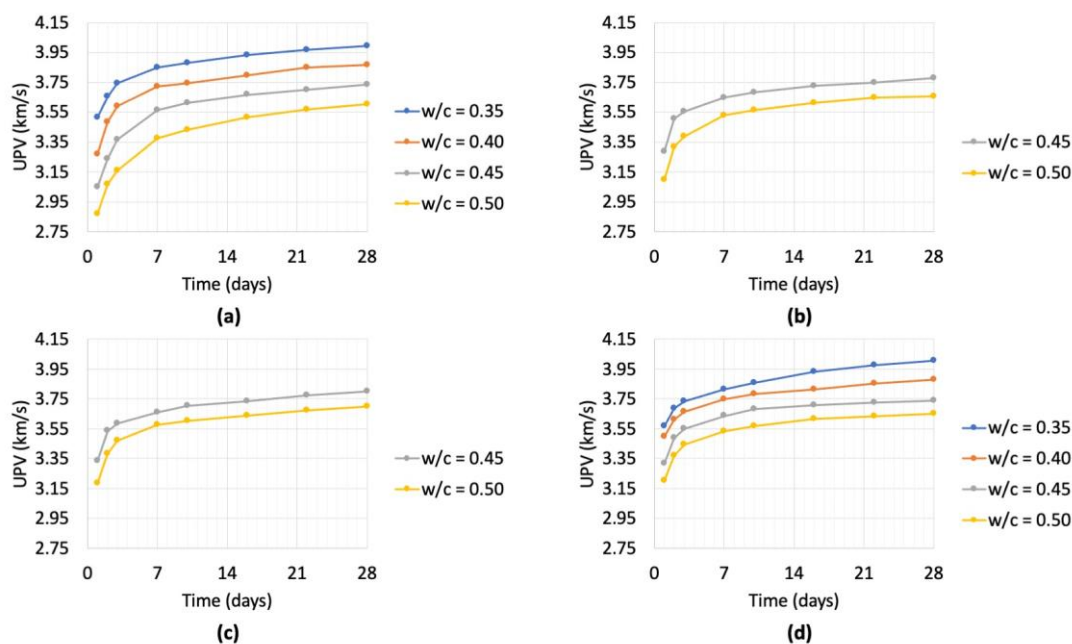
Figure 1. Ultrasonic pulse velocity of seawater-cement paste specimens with mixing water salinities of: (a) 0 g/L; (b) 12 g/L; (c) 24 g/L; (d) 36 g/L.
