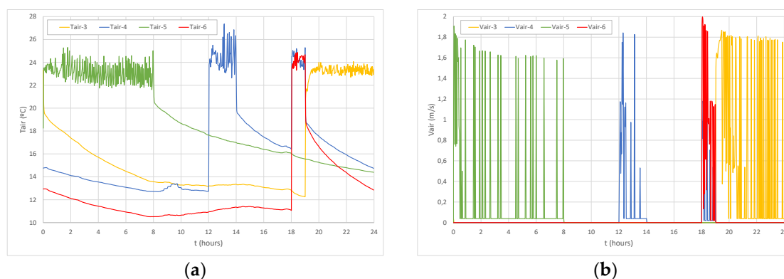
Figure 2. Evolution of (a) Tair; (b) Vair for the spaces 3, 4, 5 and 6, for the Case A.
