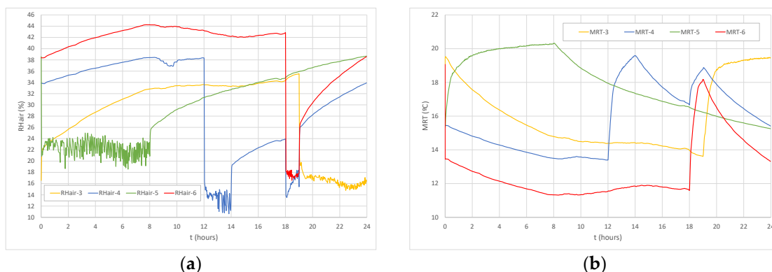
Figure 3. Evolution of (a) RHair; (b) MRT for the spaces 3, 4, 5 and 6, for the Case A.
