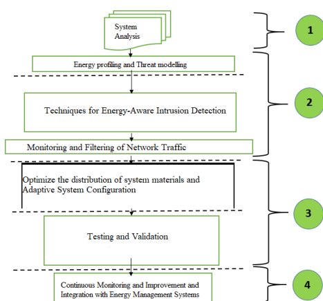
Figure 1. Methodology flow.
