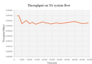
Figure 2. Throughput flow of time 10-50ms on 5G.
