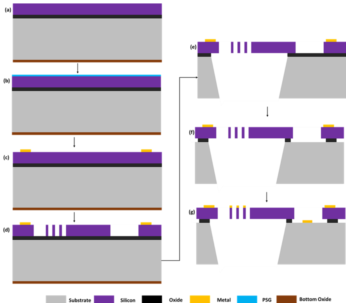
Figure 3. An overview of SOIMUMPs process (a) starting substrate SOI (b) doped silicon with Phosphosilicate glass (PSG) (c) development metal pads material (d) Silicon structural layer patterned (e) etched with DRIE (f) removal of exposed oxide layer (g) metal deposited on the structural layer.
