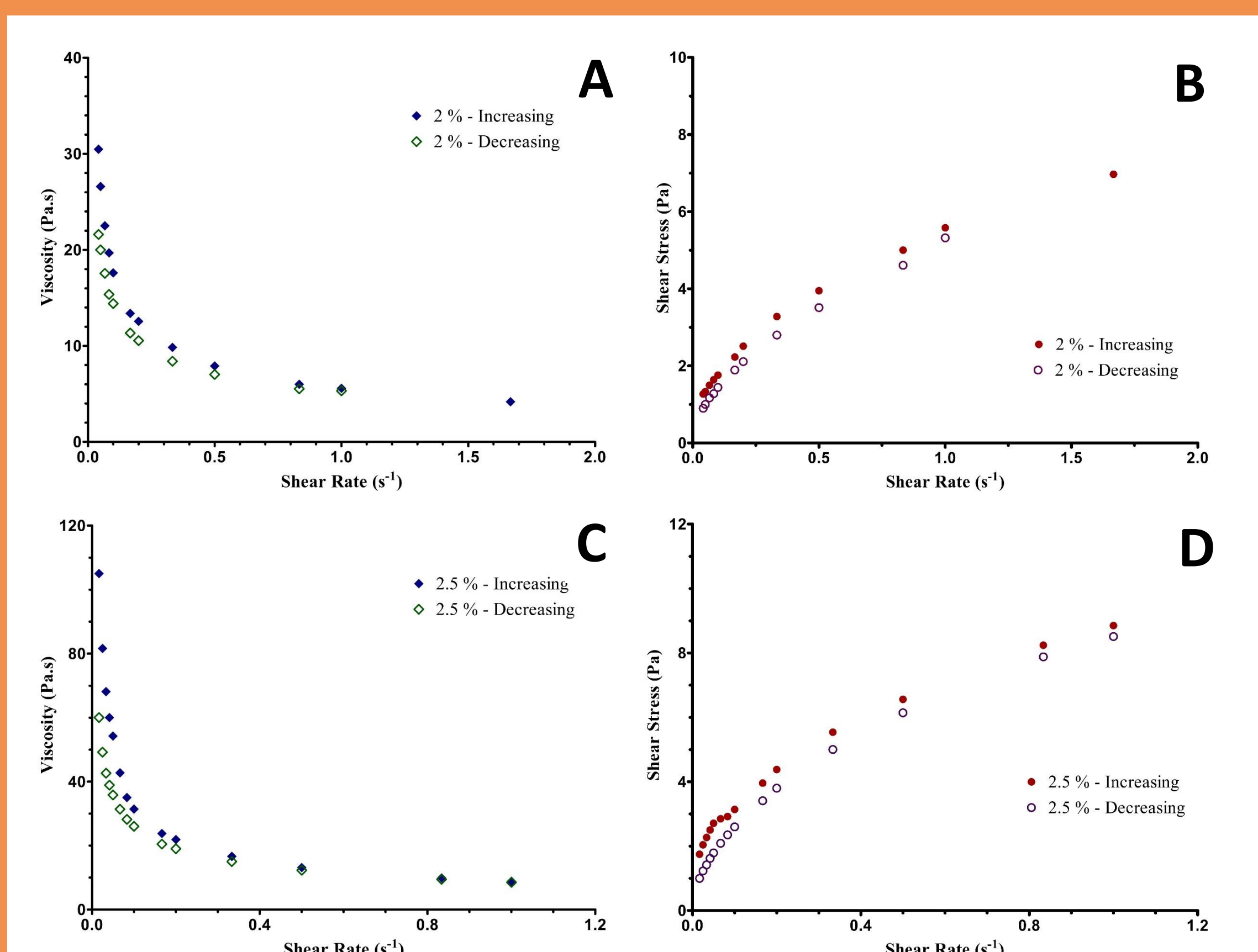
Figure 2. Viscosity as a function of shear rate for 2 wt% (A) and 2.5 wt% (C) of chitosan and Shear stress in function of shear rate for 2 wt% (B) and 2.5 wt% (D) of chitosan
