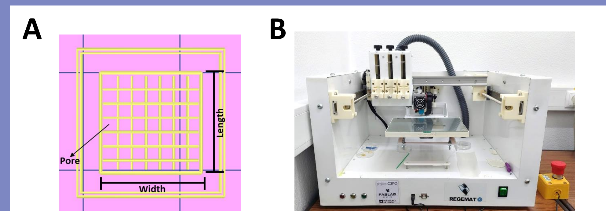
Figure 1. Scaffold CAD model (1 x 10 x 10 mm) (A) and Regemat 3D Bioprinter (B).
