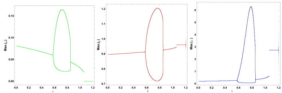
Figure 1. Dynamical changes of model(2) at refuge \psi = 0.5
