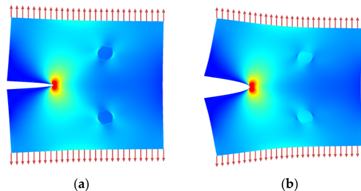
Figure 2. Von Mises stresses.
