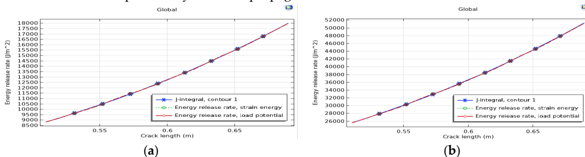
Figure 3. Energy release rates and J-integral as a function of crack length.
