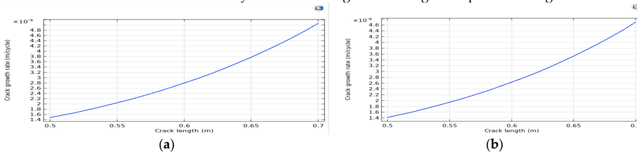
Figure 4. Crack growth rate as a function of crack length.
