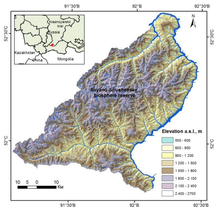
Figure 2. The study area location map.
