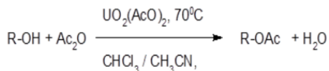
Scheme 1. Acetoxylation of alcohols with \text{Ac}_2\text{O} in the presence of Uranyl Acetate.
