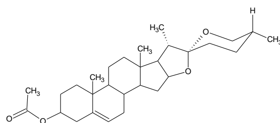
Diosgenin Acetate (m.p.: 195.80 °C/yield: 93.1%)
