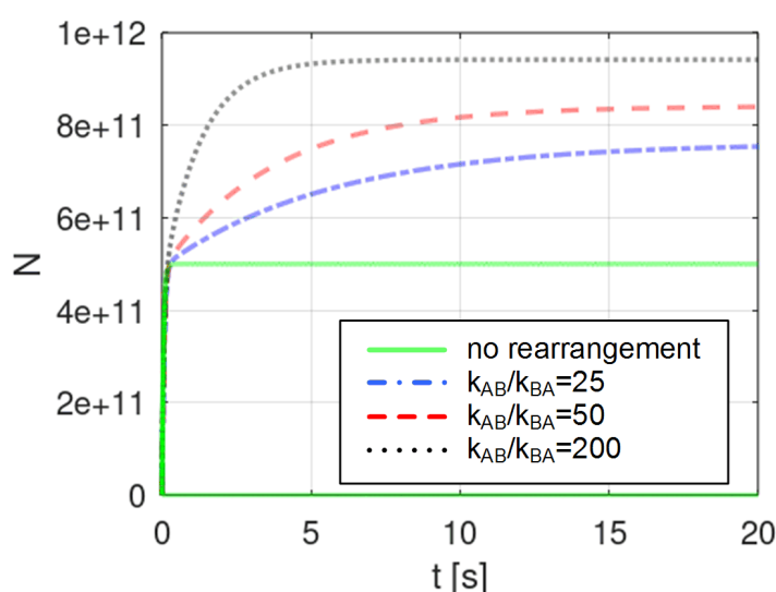
Figure 2. The time evolution of the number of adsorbed molecules, which determines the sensor response kinetics. The three cases when reversible rearrangement process occurs (with different ratios of forward and reverse rearrangement rate constants, k_{AB}/k_{BA} ) are shown, as well as the case when the configuration of biomolecules does not change after adsorption.
