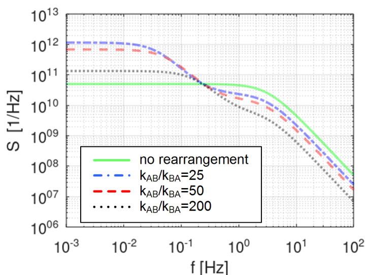
Figure 3. The power spectral density of fluctuations of the number of adsorbed biomolecules, representing the noise spectrum. The same cases are shown as in Figure 2.
