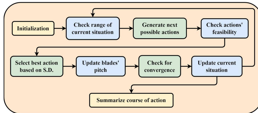
Figure 1. Workflow of the proposed blade alignment-recommender system.
