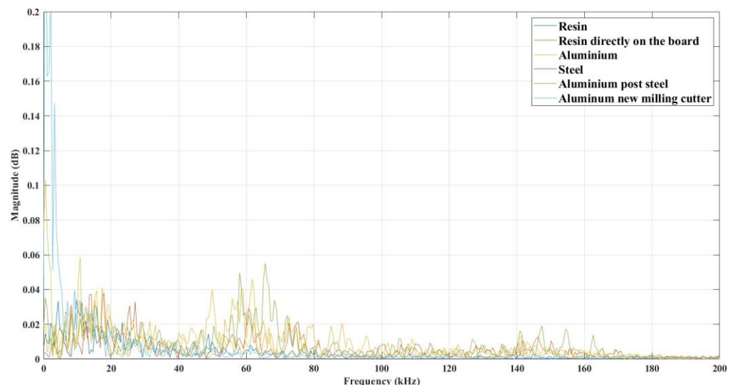
Figure 4. FFT of the main AE signals studied, in the range of 0 to 200 kHz.
