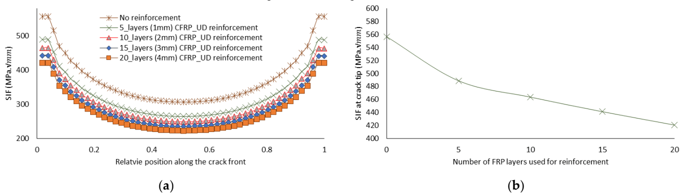
Figure 6. SIF variation due to FRP reinforcement (for a crack at saddle position, major diameter = 10 mm, minor diameter = 5 mm, reinforcement = CFRP oriented orthogonal to weld, mechanical properties [29]): (a) SIF variation along the crack; (b) SIF at the crack tip.
