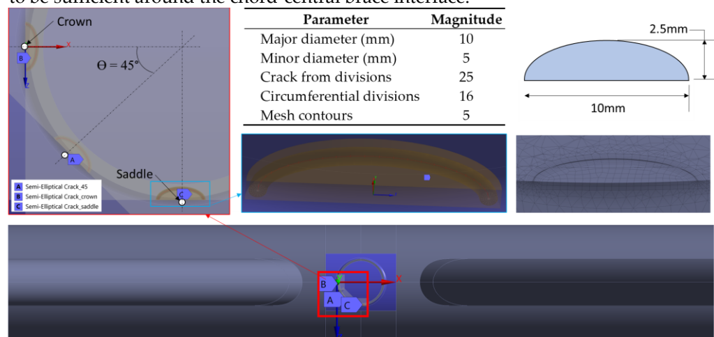
Figure 3. KT-joint with semi-elliptical crack.
