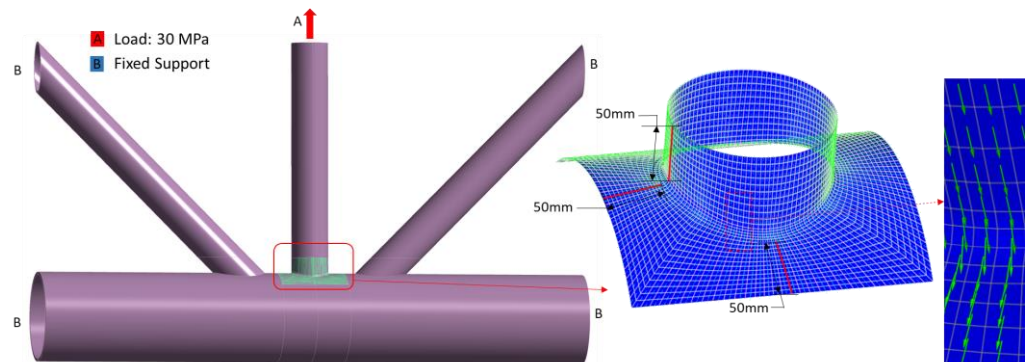
Figure 2. KT-joint with a crack at the chord and central brace interface, reinforced with CFRP UD.
