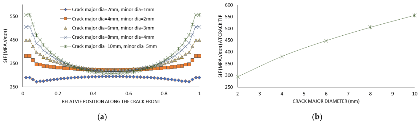
Figure 4. SIF variation with crack size (for a crack at the saddle position without reinforcement): (a) SIF along the crack front; (b) SIF at the crack tip.
