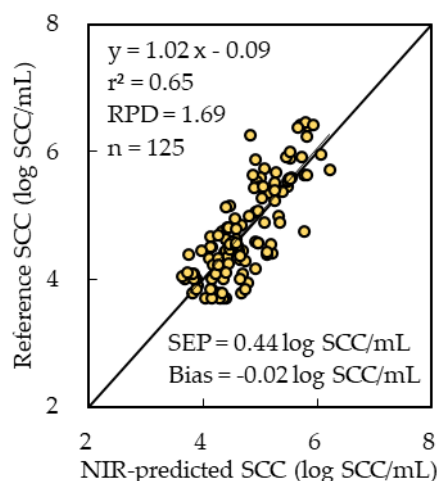
Figure 5. Correlation between reference SCC and NIR-predicted SCC at every 20 seconds during milking.
