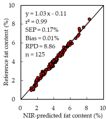
Figure 4. Correlation between reference fat content and NIR-predicted fat content at every 20 seconds during milking.
