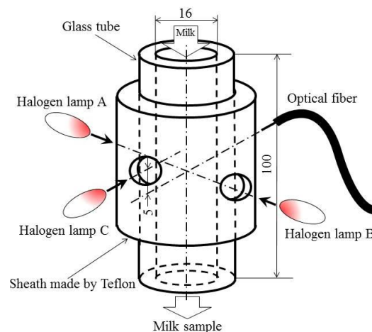
Figure 2. Schematic of the optical system of milk chamber of the near-infrared spectroscopy sensor.
