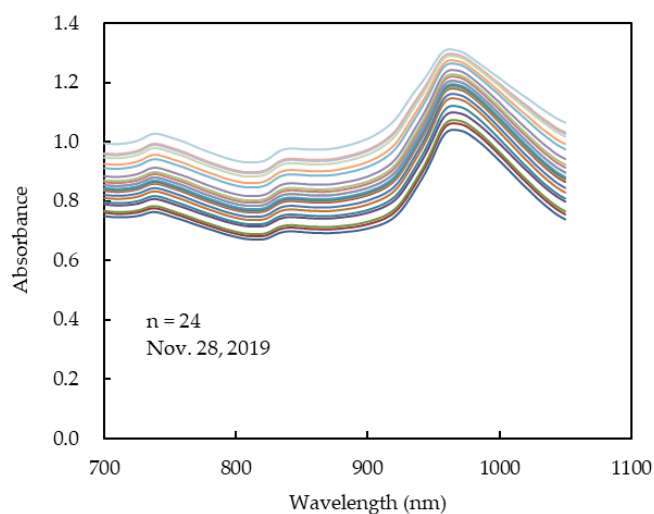
Figure 3. Original spectra of raw milk from cow number 1 during milking on November 28, 2019.
