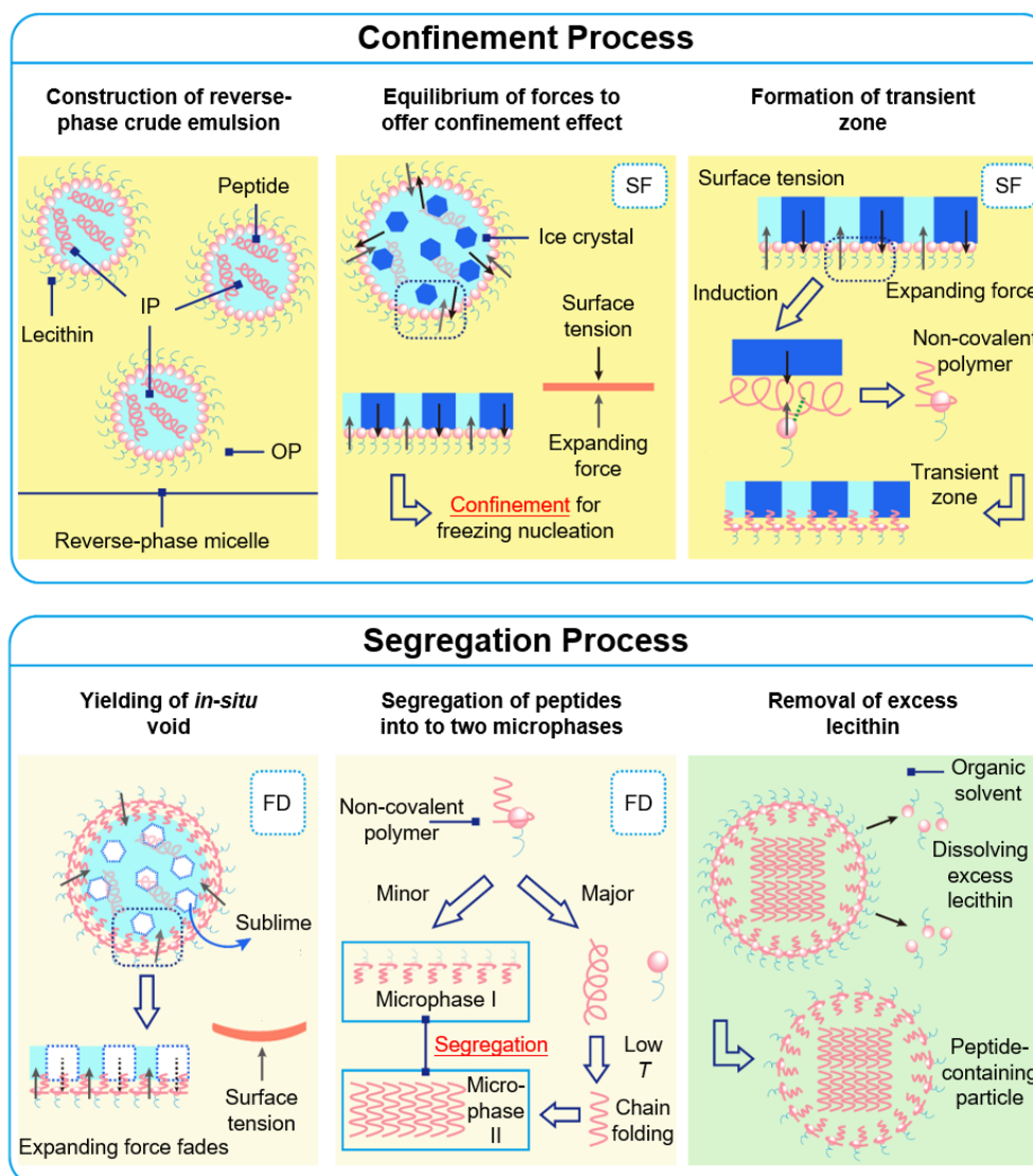
Figure 1. Scheme for confinement-segregation theory. Definition of abbreviations: IP, inner phase; OP, outer phase; SF, snap freezing; FD, freeze drying; T, temperature.
