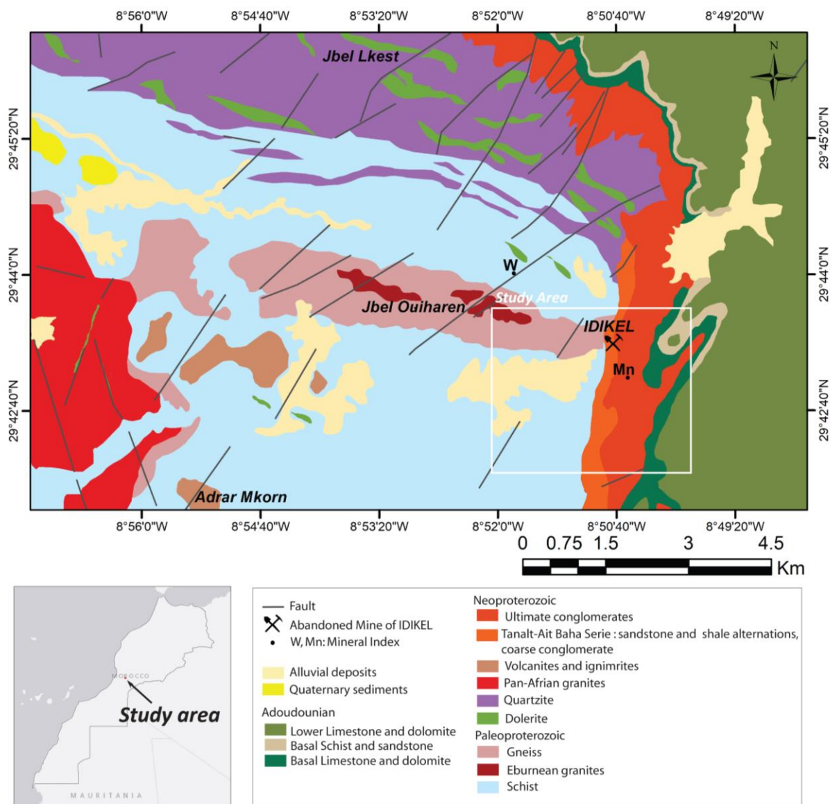
Figure 1. Geological map of the Ameln Valley area [9].
