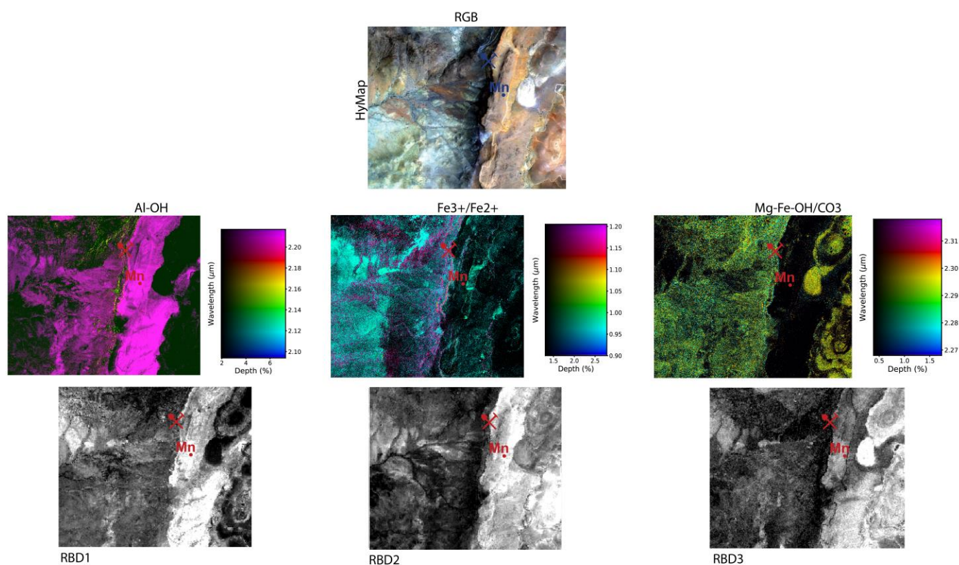
Figure 2. The results of the wavelength mapping and relative absorption band depth for the three targeted hydrothermal alteration features (i.e., Al-OH, Fe 2+ /Fe 3+ , and Mg-Fe-OH/CO 3 , from the left to the right) in the study area.
