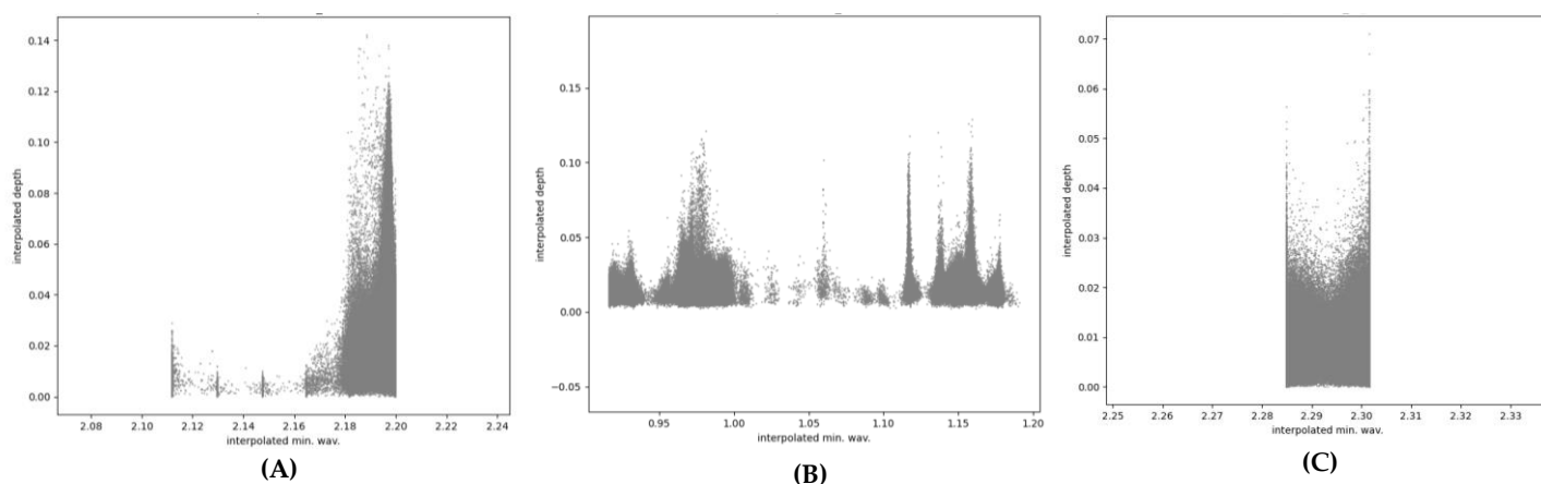
Figure 3. The plot of the absorption features depth as a function of the wavelength position for each result of the wavelength mapping for Al-OH (A), Fe 2+ /Fe 3+ (B), and Mg-Fe-OH/CO 3 (C) hydrothermal alteration minerals.
