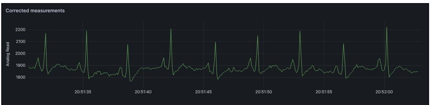
Figure 12. Grafana, low-cost ECG Corrected measurements, panel.
