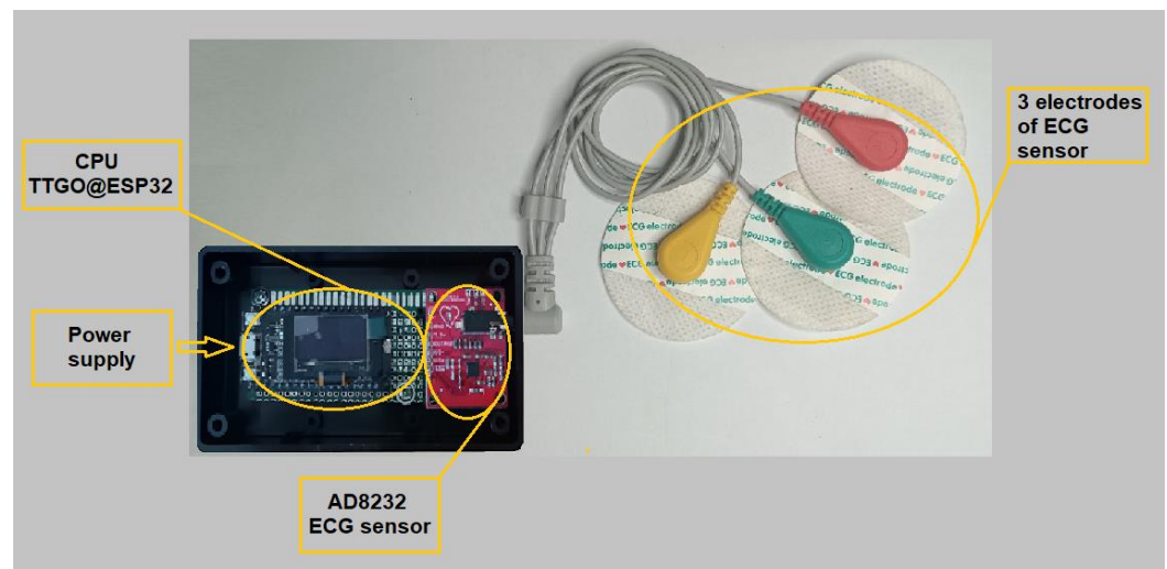
Figure 4. The complete construction of the low-cost electrocardiograph.
