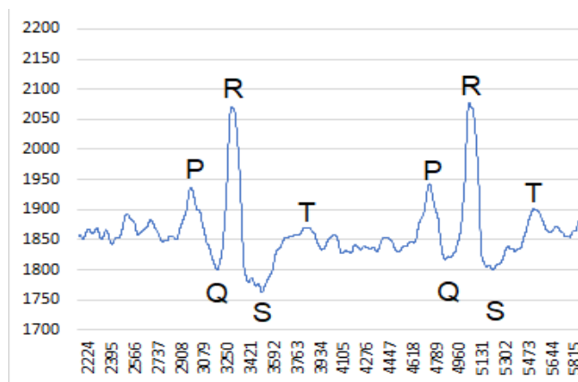
Figure 9. Time section of corrected measurements and P, Q, R, S, T points.
