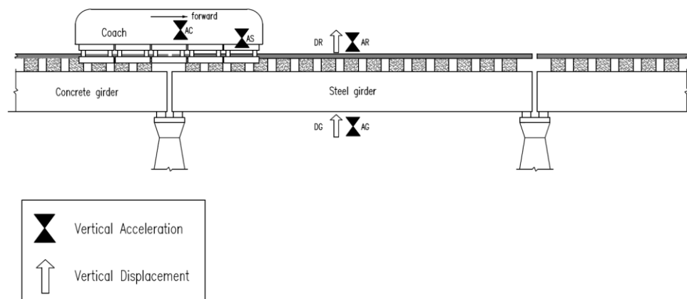
Figure 5. Test set-up and measurement points layout.
