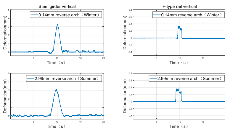
Figure 6. Deformation of steel girder and F-type rail: comparison between the data collected in Winter (top row) and Summer (bottom row).
