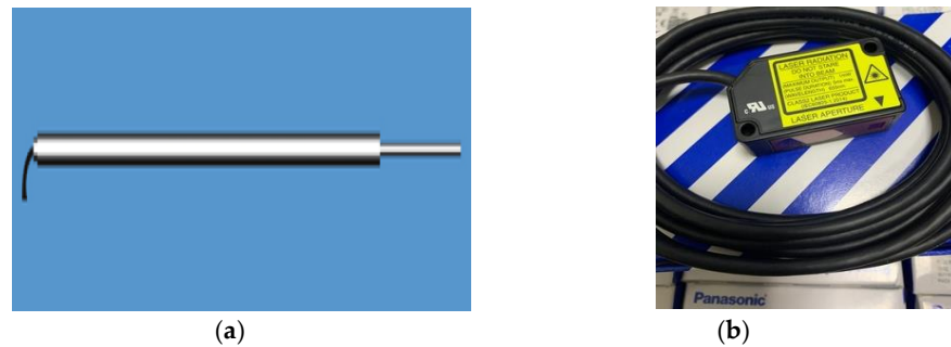
Figure 2. Adopted displacement sensors: (a) Keyu LVDT-WYDC contact displacement sensor; (b) Panasonic HG-C1030 laser displacement sensor.
