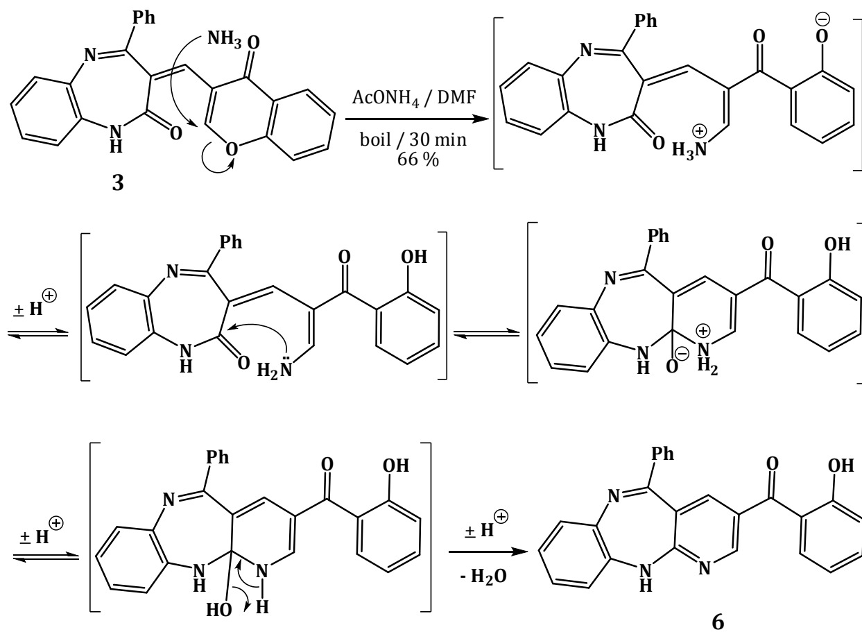
Scheme 3. Rearrangement of compound 3 into pyridobenzodiazepine 6 .
