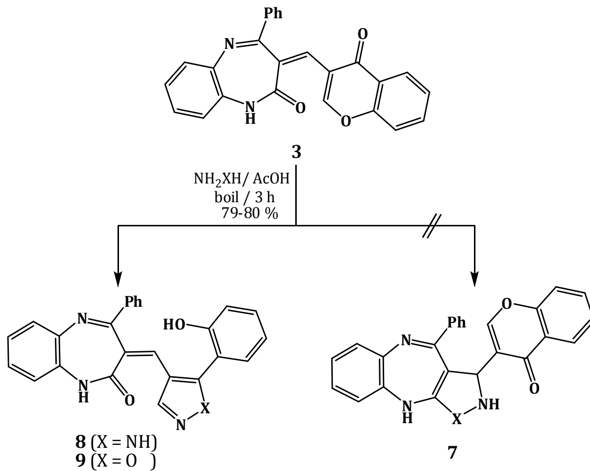
Scheme 4. Reaction of compound 3 with hydrazine and hydroxylamine.
