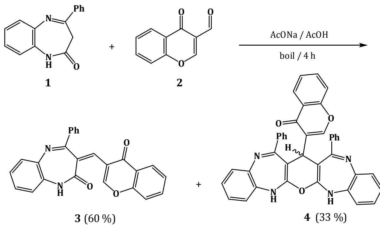
Scheme 1. Reaction of 4-phenyl-1H-[1,5]benzodiazepin-2(3H)-one ( 1 ) with 3-formylchromone ( 2 ).
