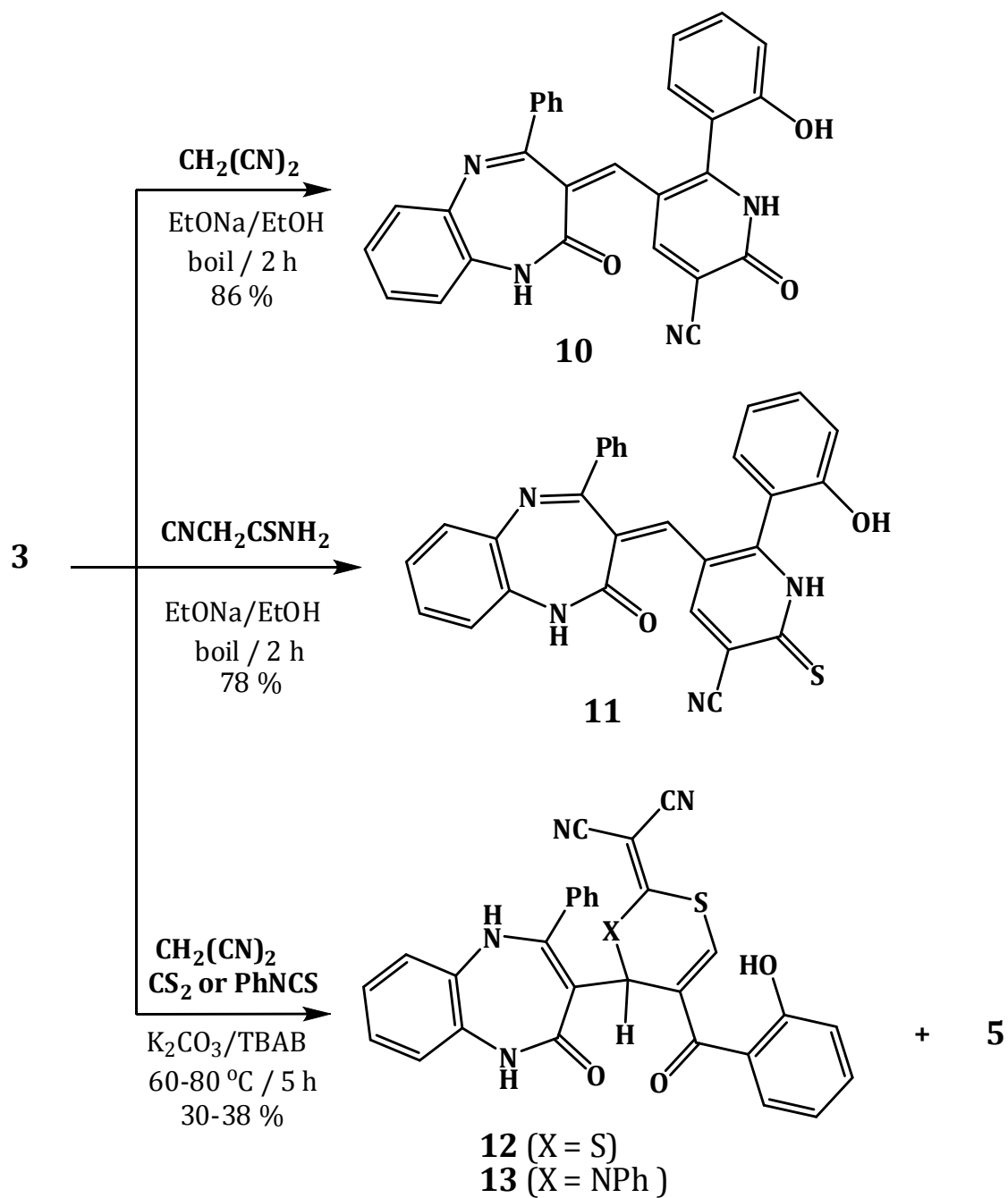
Scheme 5. Reaction of compound 3 with some 1,3-binucleophiles.
