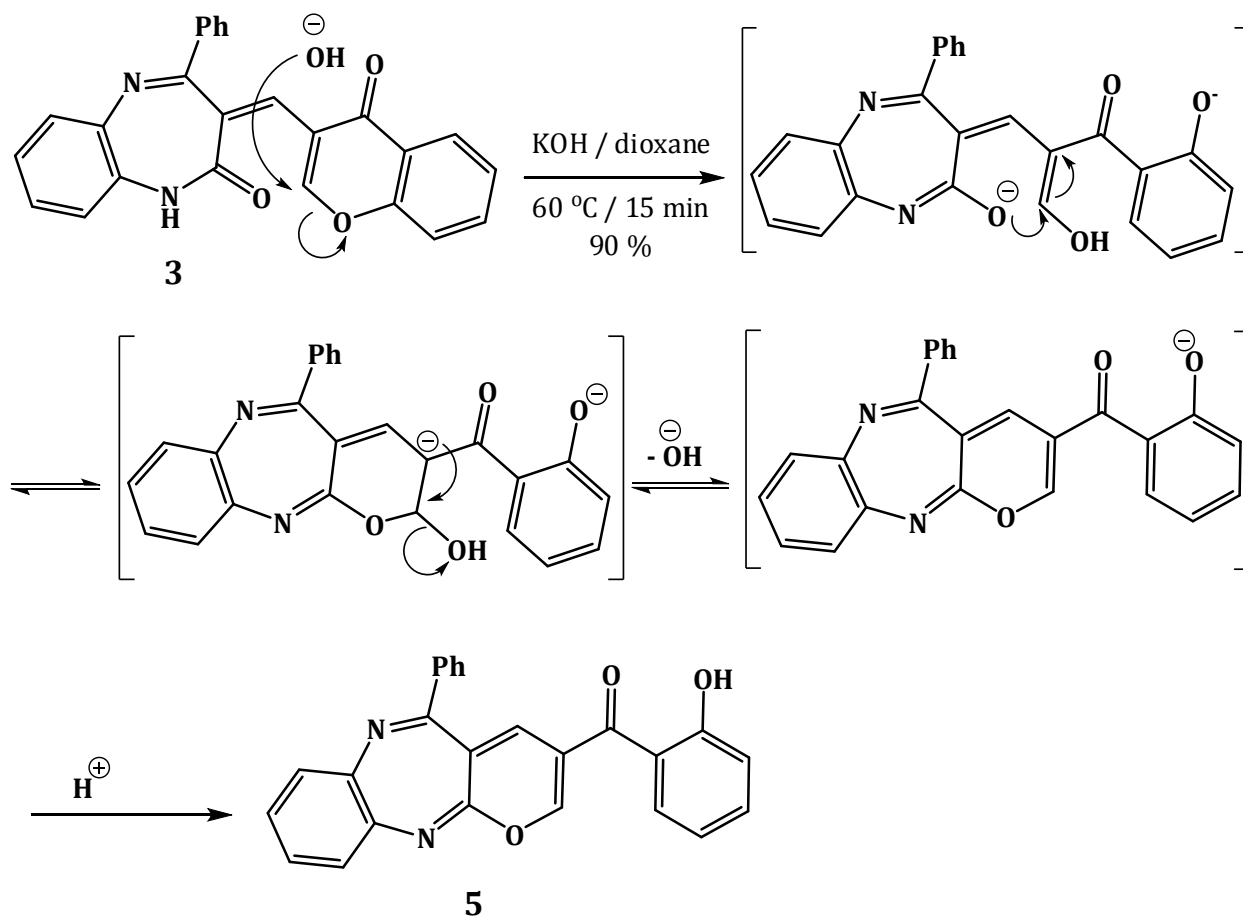
Scheme 2. Rearrangement of compound 3 into pyranobenzodiazepine 5 .
