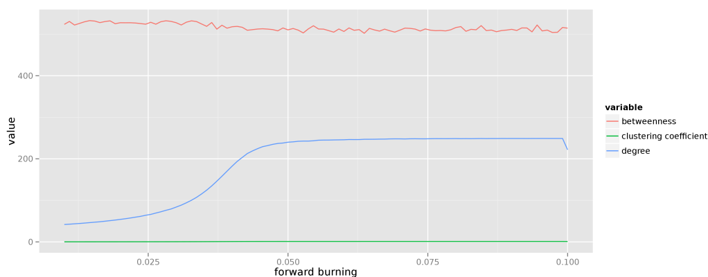
Figure 4. Centrality measures for forest fire graphs
