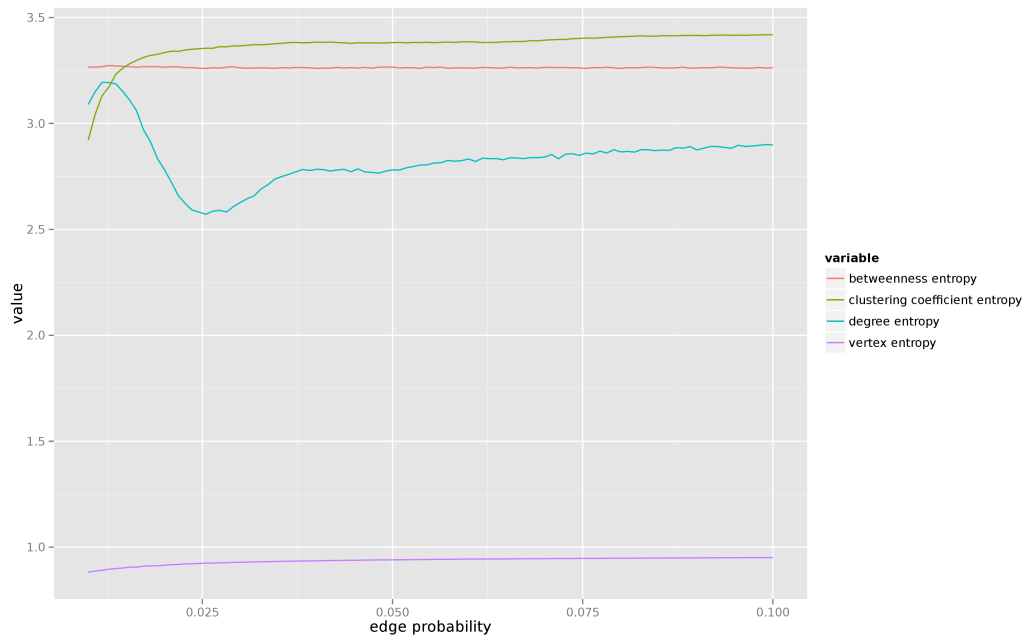
Figure 5. Entropy of centrality measures for random graphs
