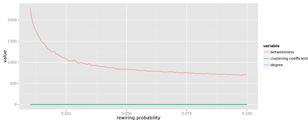
Figure 2. Centrality measures for small world graphs
