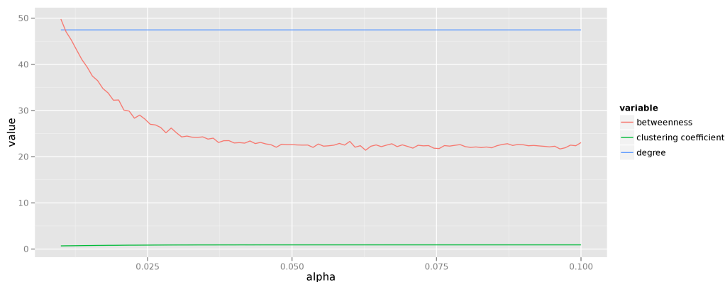
Figure 4. Centrality measures for forest fire graphs
