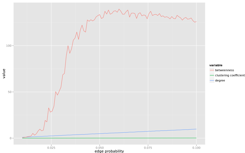
Figure 1. Centrality measures for random graphs
