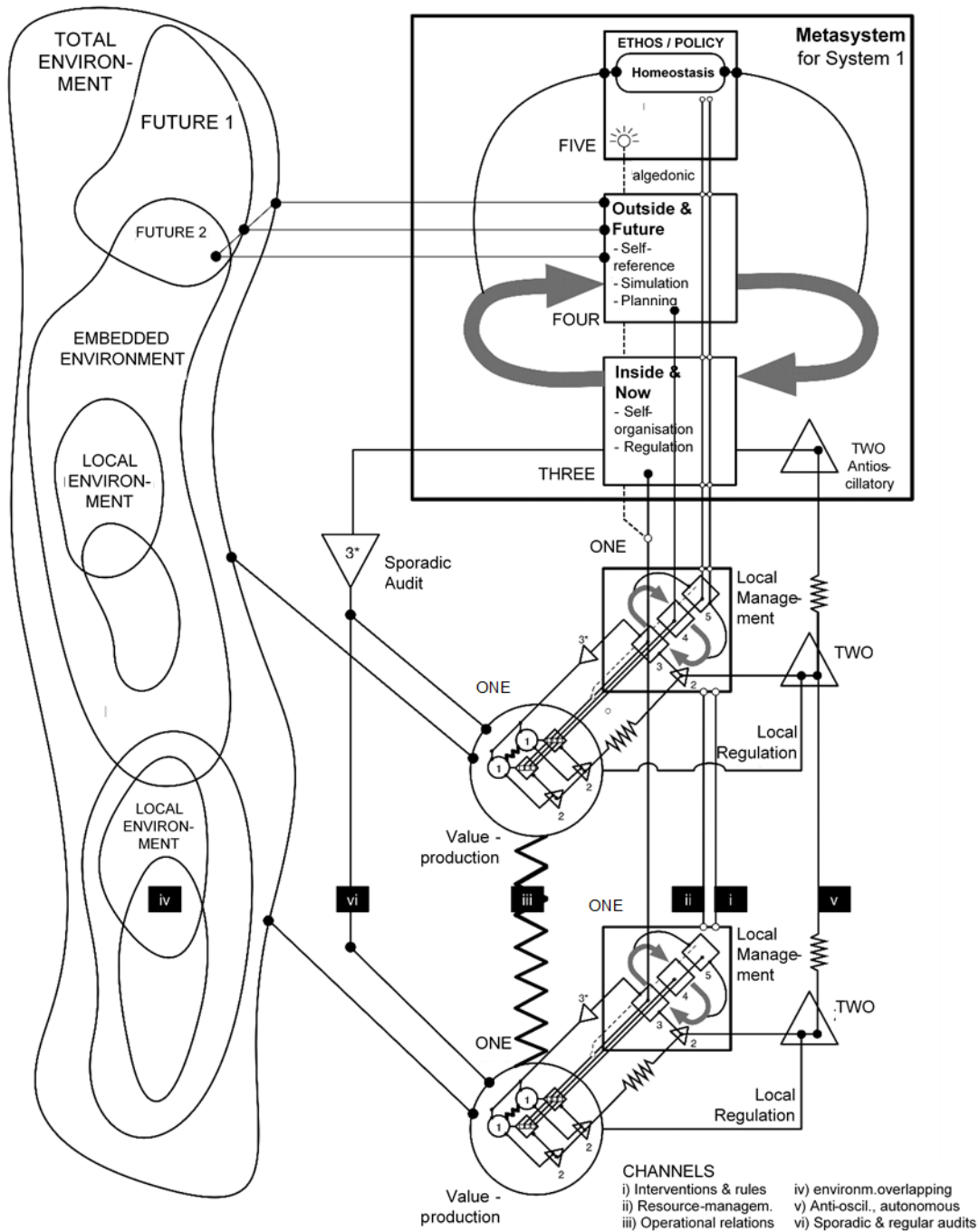
Figure 1. Stafford Beer’s Viable System Model (cyber-subidiarity) for any sustainable organization. Its recursiveness is explicitly represented in System 1. System 3* correspond to an extension of System 3 to enhance its knowledge about System 1 performance in order to provide a better regulation. (Illustration elaborated from [6])
