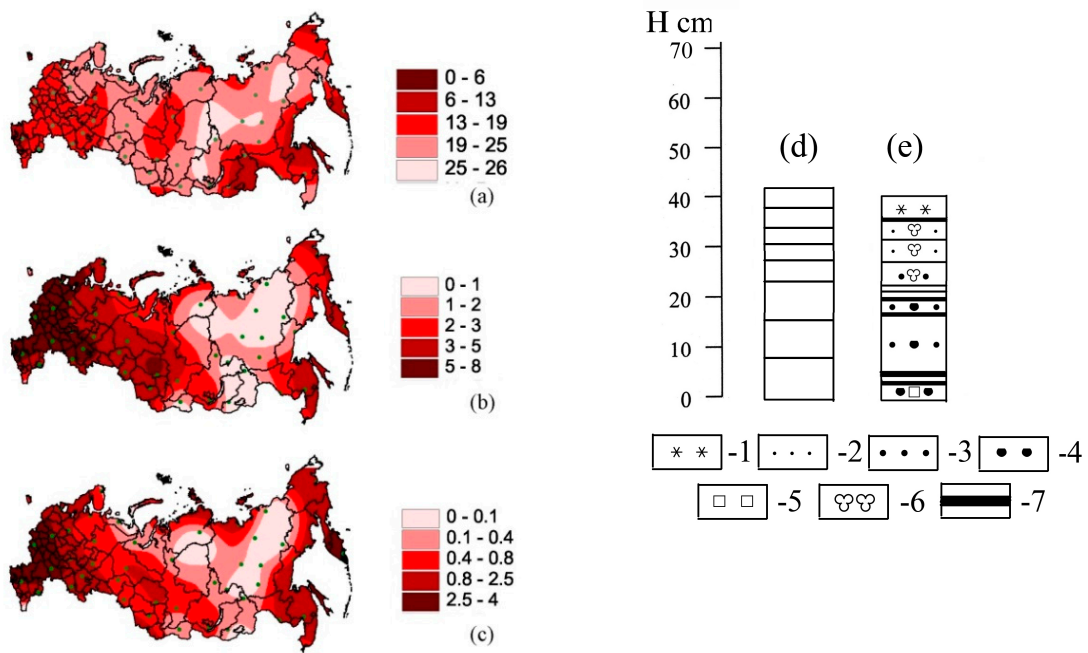
Figure 1. Number of snowfalls for the averaged winter period with intensity: (a) - 0.1 – 2.5 mm; (b) - 2.5-5 mm; (c) - 5-10 mm. Moscow region stratigraphic columns for the maximum of snow accumulation: (d) – modeled, generalized-averaged for winter seasons 1960-2016; (e)– real observations for winter season 2014/15. Snow stratigraphy notation: (1) – new snow; (2) – fine-grained snow; (3) – medium-grained snow; (4) – coarse-grained snow; (5) – faceted crystals; (6) – refrozen ice crystals; (7) – ice crust.
