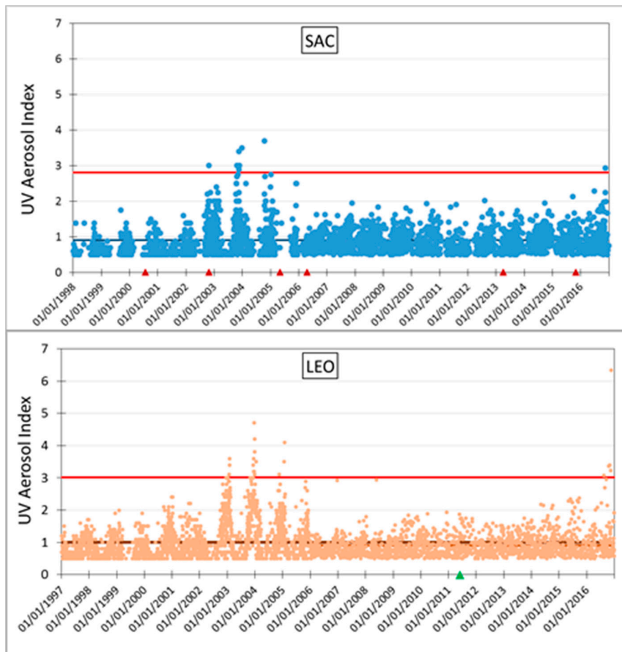
Figure 5. Top. UV aerosol index measured by TOMS and OMI instruments on board of different NASA satellites, at the SAC site. The red arrows indicate the days when a significant eruption was produced by the near Lascar volcano. Bottom: similar results for LEO site, with a green arrow indicating the day of large eruption originated in the Puyehue-Cordón Caulle volcanic complex. The horizontal line in the middle of the data indicates the mean value. Goddard Space Flight Center/NASA https://science.nasa.gov/missions/toms .
