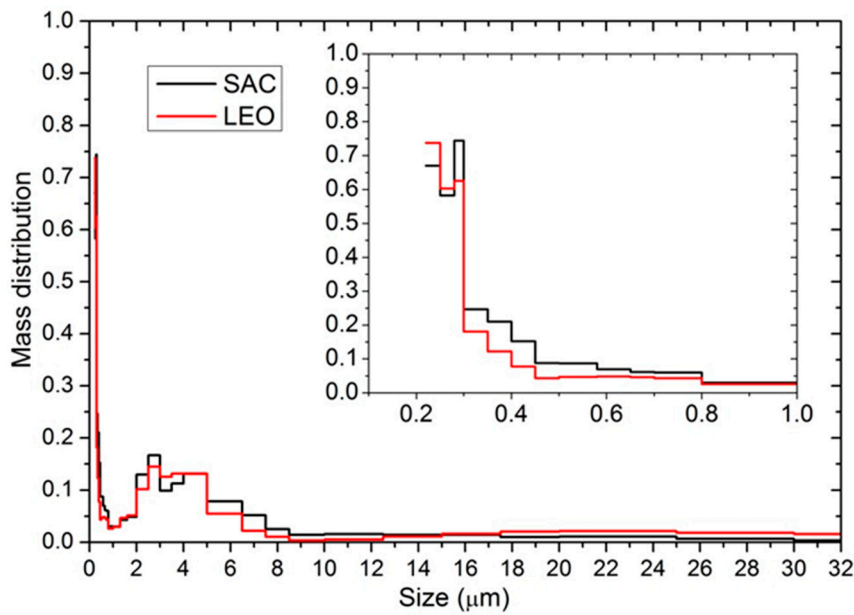
Figure 2. Normalized mean mass concentration distribution for SAC site (black line) and LEO site (red line).
