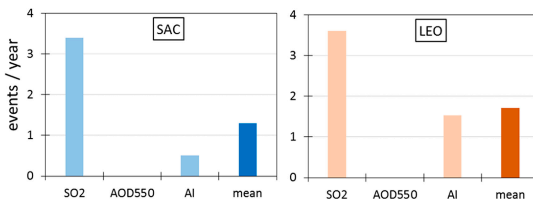
Figure 8. Comparison between the frequency of events from different sources of data (SO 2 total column, AOD 550 or AI), and mean value, for the SAC and LEO sites.
