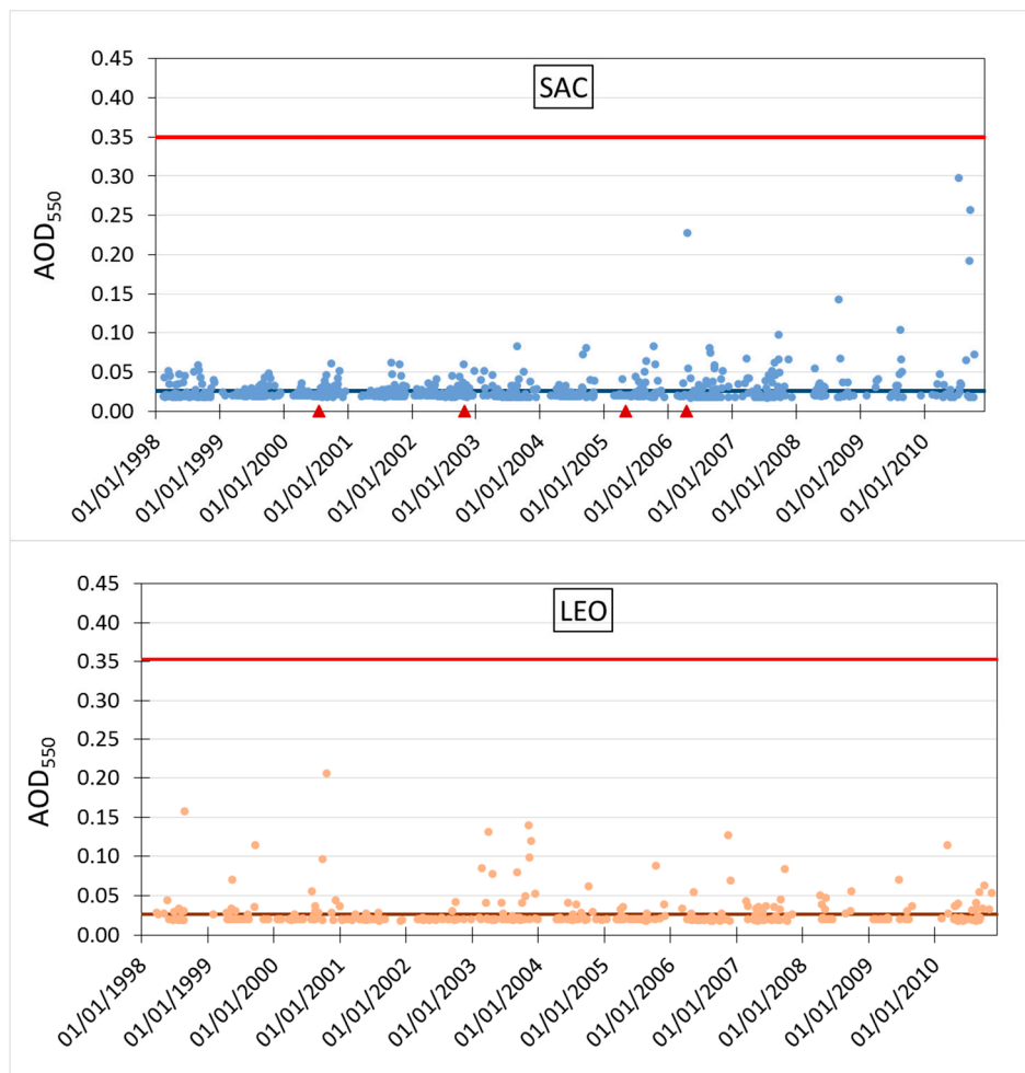
Figure 7.Top. Aerosol optical depth at a wavelength of 550 nm (AOD 550 ) measured by SeaWiFS instrument on board of SeaStar/NASA satellite, for SAC site, in the 1998-2010 period. The days with significant eruptions of the Lascar volcano (20-07-2000, 26-10-2002, 04-05-2005 and 18-04-2006) are indicated with red arrows on the horizontal axis. The horizontal line in the middle of the data indicates the mean value. Bottom: similar results for LEO site. Source: Goddard Space Flight Center/NASA. https://www.nasa.gov/goddard .
