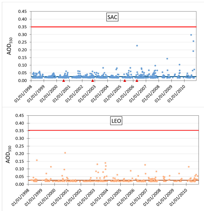
Figure 4. Area average ( 1^\circ \times 1^\circ ) time series (1998-2010 period) aerosol optical depth at 550 nm ( AOD_{550} ) for SAC and LEO sites. The mean values are: AOD_{550,SW,SAC}^* = 0.0262 ( \sigma_P = 0.161 ) for SAC (top figure) and AOD_{550,SW,LEO}^* = 0.0266 ( \sigma_P = 0.161 ) for LEO (bottom figure). The red line corresponds to the limiting value given by formula (1). Note: in the top figure, the red arrows indicate the Lascar volcano eruption days: 20-07-2000, 26-10-2002, 04-05-2005 and 18-04-2006. Source: SeaWiFS instrument on SeaStar/NASA satellite Deep Blue Level 3 long-term aerosol data at http://disc.sci.gsfc.nasa.gov/giovanni/ .
