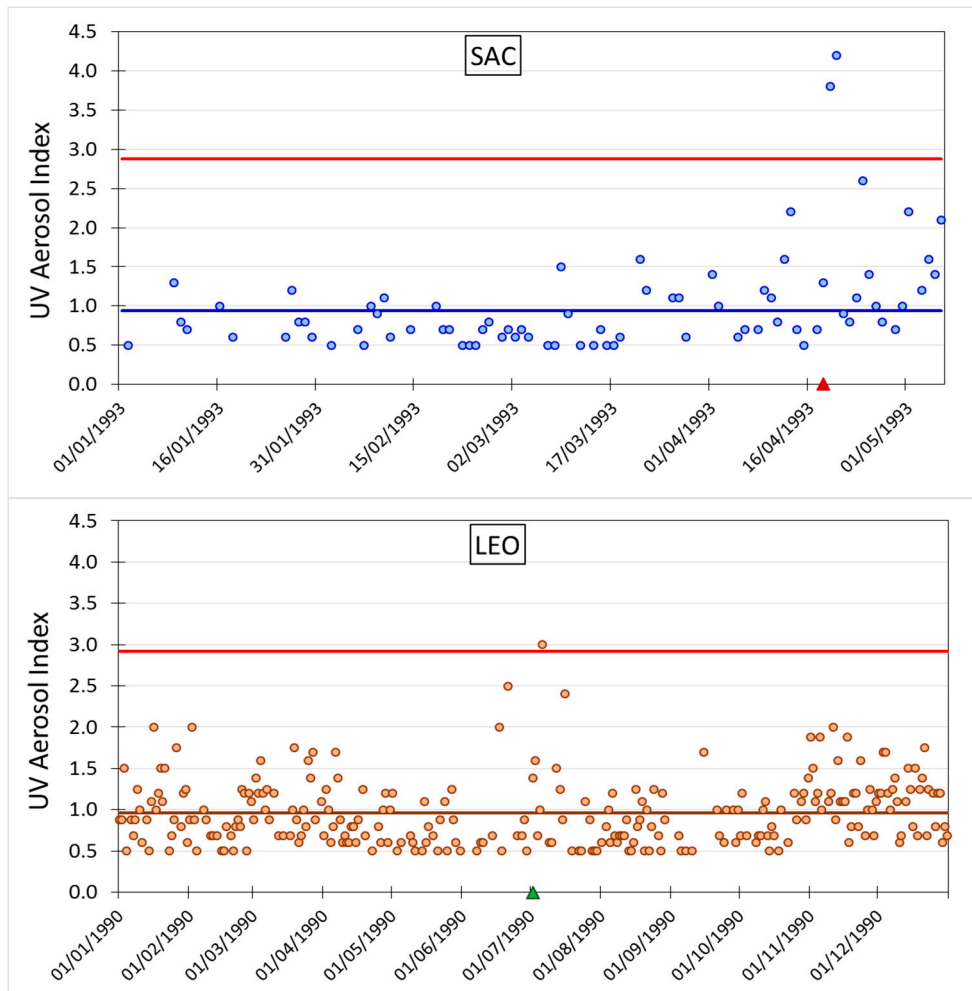
Figure 6. Top. UV aerosol index measured by TOMS instrument onboard Nimbus-7 NASA satellite, at the SAC site. The red arrow indicates the day 18 April 1993 when a significant eruption was produced by the near Lascar volcano. Bottom: similar results for LEO site, with a green arrow indicating the day 2 July 1990 of a large eruption produced by the Puyehue-Cordón Caulle volcanic complex. The horizontal line in the middle of the data indicates the mean value. Source. Goddard Space Flight Center/NASA.
