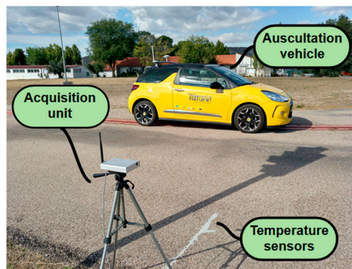
Figure 7. Overall view of the dynamic test.
