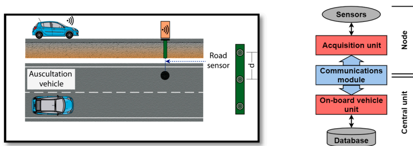
Figure 1. Conceptual diagram of the proposed monitoring systems including the main subsystems.
