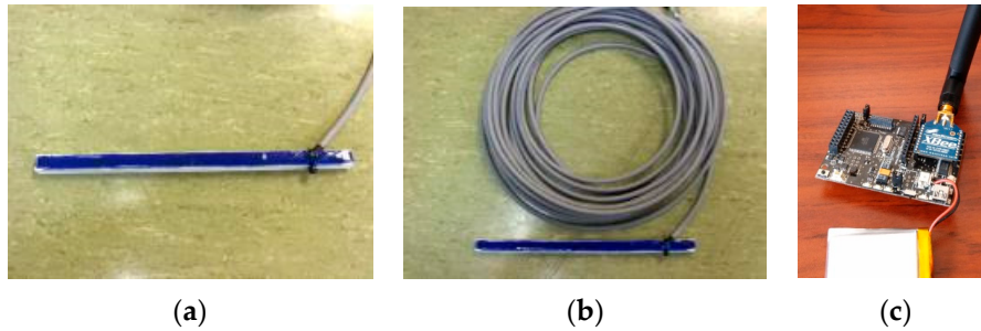
Figure 2. (a) DS18B20 support; (b) node sensors set; (c) Libelium Waspote with XBEE module.
