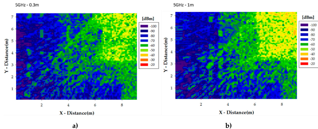
Figure 3. Bi-dimensional received power level distributions at an operating frequency of 5.8GHz, for h=0.3\text{m} (a) and h=1\text{m} (b)
