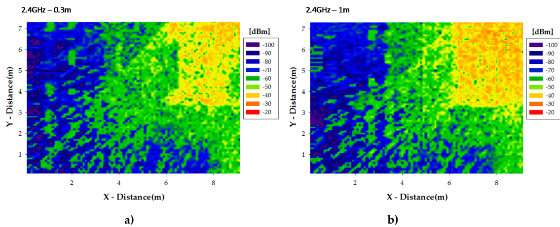
Figure 2. Bi-dimensional received power level distributions at an operating frequency of 2.4GHz, for h=0.3\text{m} (a) and h=1\text{m} (b)
