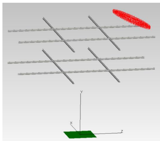
Figure 2. TracePro model constituted of the measurement plane (green), the supporting frame (grey) and the lighting system (red) for the 3x3 scenario with an incident angle of 24°
