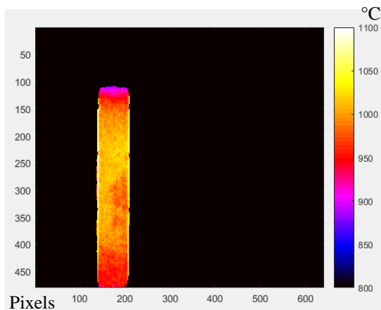
Figure 5: Temperature field measurement
