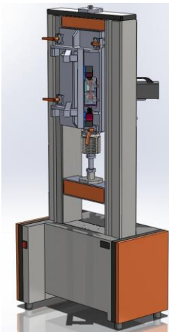
Figure 1: Machine overview
