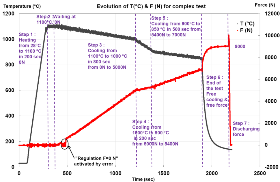
Figure 7: Complex test with load and temperature PID monitoring
