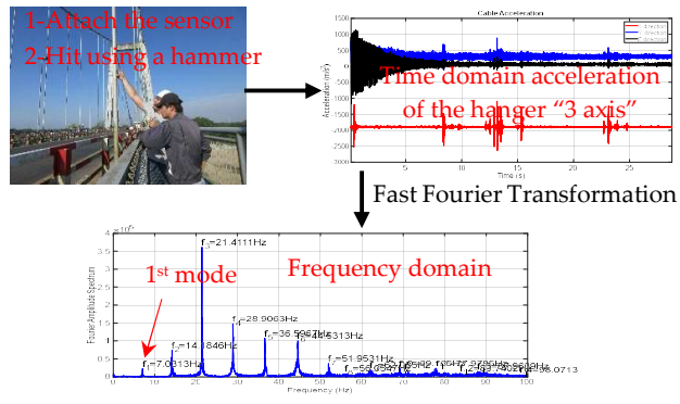
Figure 6. Measurements' procedure
