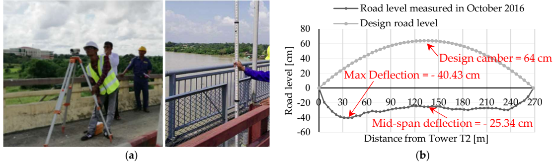
Figure 4. (a) During the measurement of road level; (b) Design road level and measured road level.
