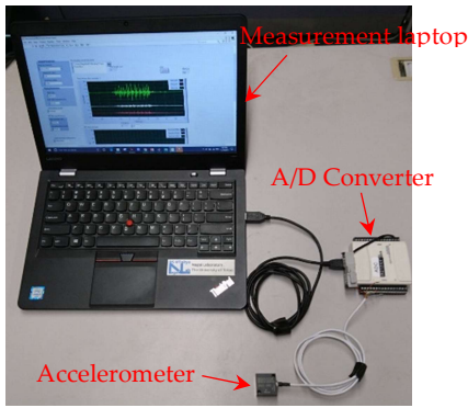
Figure 5. Measurements' system
