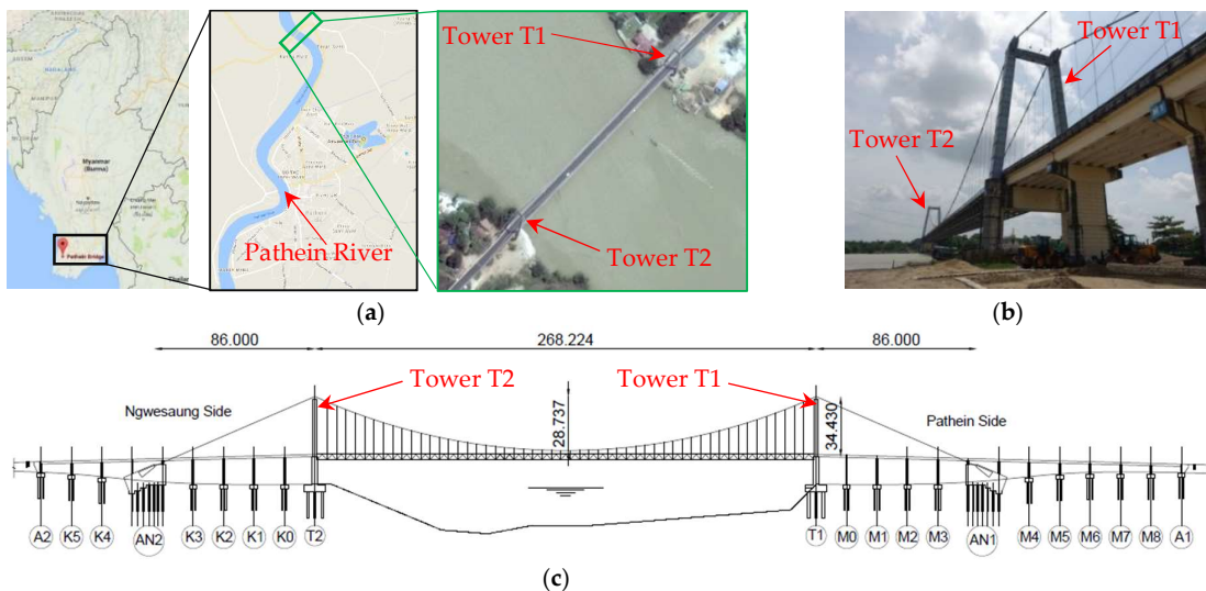
Figure 2. Pathein bridge. (a) Location of the bridge on Myanmar's map; (b) Picture of the bridge; (c) Elevation of the bridge as per design drawings.
