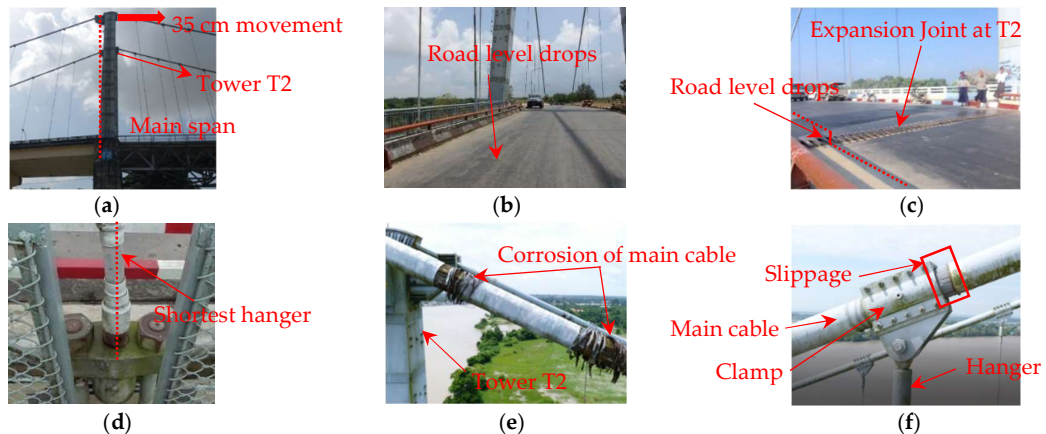
Figure 3. The damages in Pathein bridge. (a) Inclination of tower T2; (b) Road level sinking down; (c) Road level drops down after the bearing failed; (d) Inclination of hangers; (e) Corrosion of the main cable; (f) Slippage of clamps.
