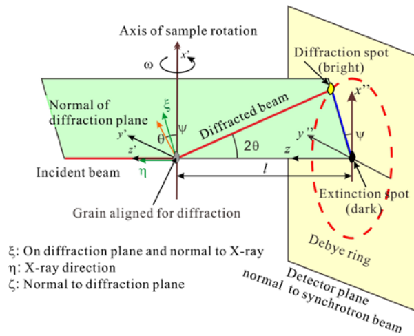
Fig. 1. Principle of DCT.
