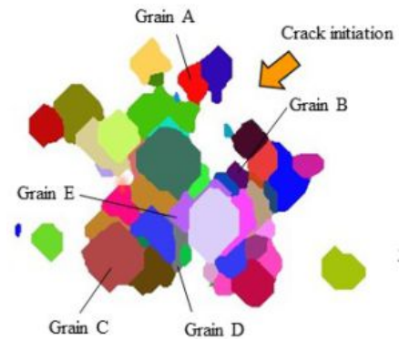
Fig. 4. Cross section of specimen at crack initiation site.
