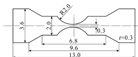
Fig. 2. Shape and dimensions of specimen.
