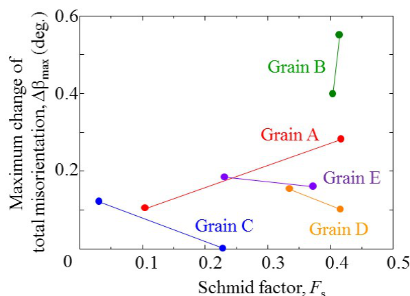
Fig. 6. Effect of Schmid factor on maximum change of total misorientation, \beta , in fatigue.
