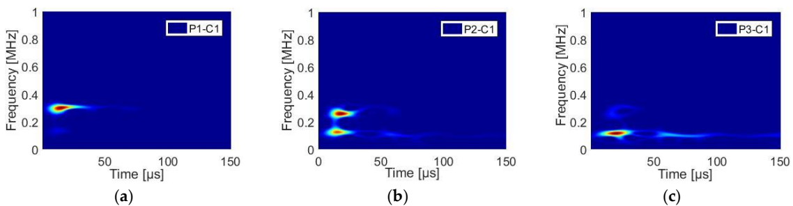
Figure 8. Time-frequency results calculated using smoothed pseudo Vigner-Ville distribution for 3 source positions for signals recorded on C1
