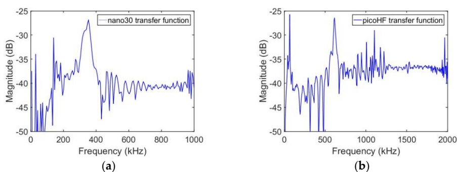
Figure 3. Transfer function of (a) nano30 and (b) picoHF, determined by reciprocity method
