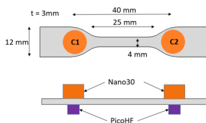
Figure 1. Dimension of specimen and sensors placement
