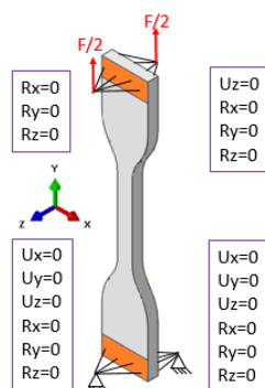
Figure 2. Scheme of the numerical specimen with the boundary conditions
