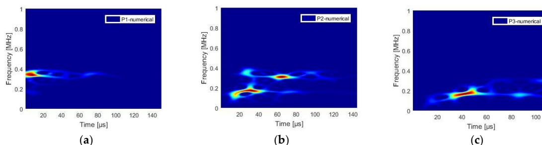
Figure 11. Numerical results: time frequency calculated smoothed pseudo Vigner-Ville distribution for three source positions.
