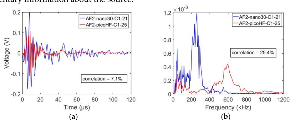
Figure 9. Temporal signals (a) and frequency spectra (b) for two 2 type of sensors
