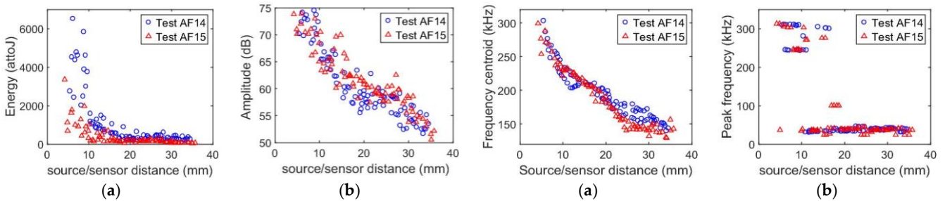
Figure 6. Temporal descriptors vs. source/sensor distance: (a) Energy in attoJ, (b) amplitude in dB
