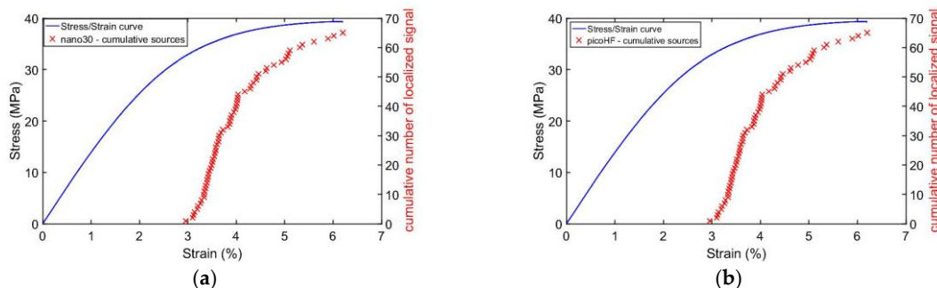
Figure 5. Cumulative localized signal during SFFT: (a) sources located by nano30; (b) by picoHF
