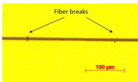
Figure 4. Fiber breaks as observed by optical microscopy
