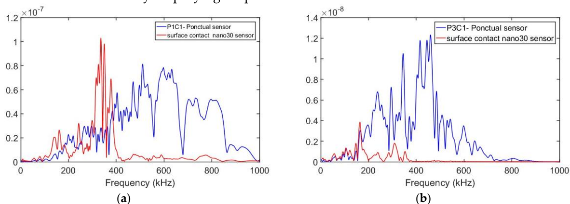
Figure 10. Comparison between simulated punctual sensors, surface contact sensors. (a) Signals of simulated fiber break at P1 position at C1 sensor; (b) at P3 position at C1 sensor
