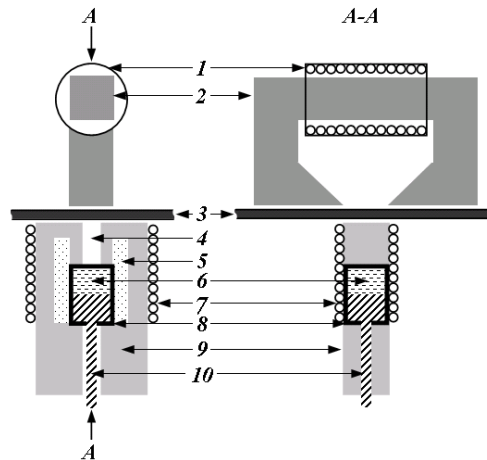
Figure 1. The growing vessel for scanning LPE: 1 – coil, 2 – magnetic conductor, 3 – substrate, 4 – growth capillary, 5 – high-temperature insulator (ceramics), 6 – solution-melt, 7 – heater, 8 – homogenization container, 9 – electrode, 10 – piston.
