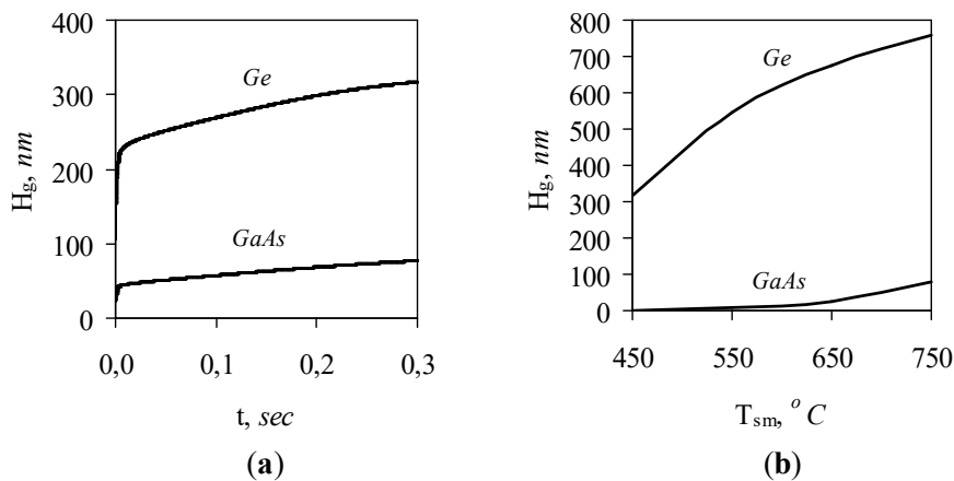
Figure 2. The dependence of maximum thickness H_g of the epitaxial layers grown on the contact time between the solution-melt and the substrate (Ge layer from Ga-Ge solution-melt, solution-melt temperature T_{sm}=450 ^{\circ}C , substrate temperature T_s=27 ^{\circ}C ; GaAs layer from Ga-As solution-melt, T_{sm}=750 ^{\circ}C , T_s=266 ^{\circ}C ) (a). The dependence of maximum thickness H_g of the epitaxial layers (Ge and GaAs) grown within 0.3 s on the solution-melt initial temperature T_{sm} (b).
