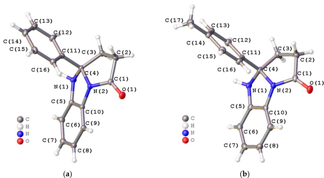
Figure 1. Crystal structure with atoms labeling of: (a) 1a; (b) 1b. Displacement ellipsoids are drawn at the 50% probability level.
