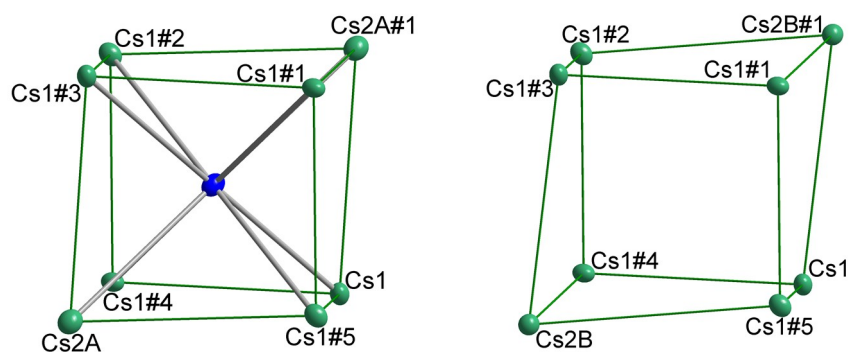
Figure 3. Distorted cubic arrangement around the halide, respectively void. Cs1: x, y, z ; Cs1#1: 1-y, x-y, z ; Cs1#2: 1-x+y, 1-x, z ; Cs1#3: 4/3-x, 2/3-y, 2/3-z ; Cs1#4: 1/3+y, 2/3-x+y, 2/3-z ; Cs1#5: 1/3+x-y, -1/3+x, 2/3-z ; Cs2A/B: x, y, z ; Cs2A/B#1: 4/3-x, 2/3-y, 2/3-z .
