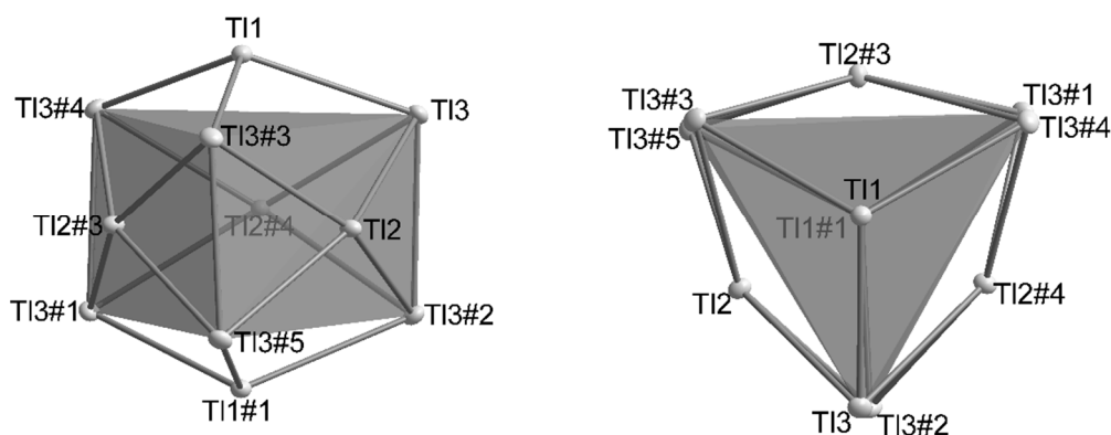
Figure 2. The distortion of the trigonal prism in the \text{Tl}_{11}^{7-} results in the point group D_3 for the cluster. Symmetry operations for the generation of equivalent atoms: #1: 1/3+x-y, 2/3-y, 7/6-z ; #2: 1/3+y, -1/3+x, 7/6-z ; #3: 1-y, x-y, z ; #4: 1-x+y, 1-x, z ; #5: 4/3-x, 2/3-x+y, 7/6-z .
