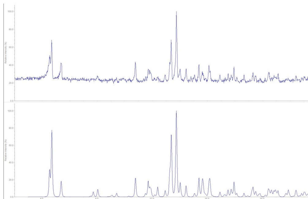
Figure 1. Powder diffraction patterns of \text{Cs}_8\text{Tl}_{11}\text{Cl}_{0.8} : Measured (top) and calculated (bottom; from single crystal data of \text{Rb}_8\text{Tl}_{11} and adapted unit cell parameters of \text{Cs}_8\text{Tl}_{11} due to missing cif-files of \text{Cs}_8\text{Tl}_{11} in the data base).
