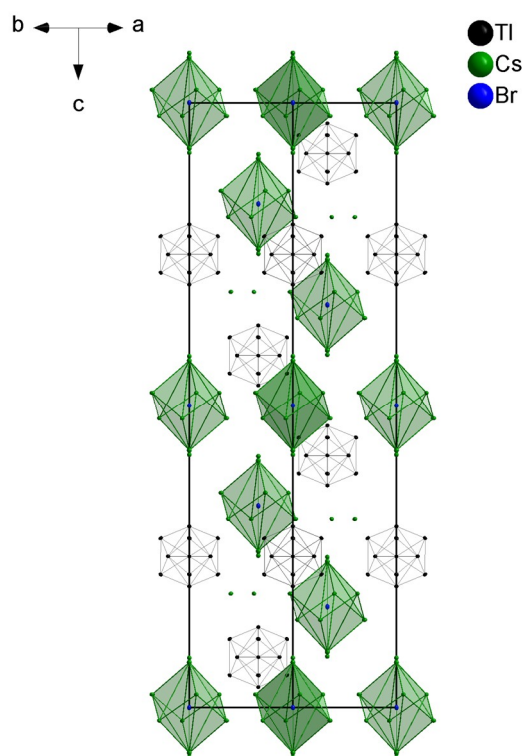
Figure. 4 The unit cell of Cs_8Tl_{11}Br_{0.9} shows the two characteristic components: Tl_{11} clusters and the distorted cubic arrangement around the halide atom.
