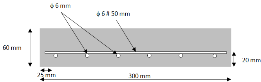
Figure 1. RC slab details
