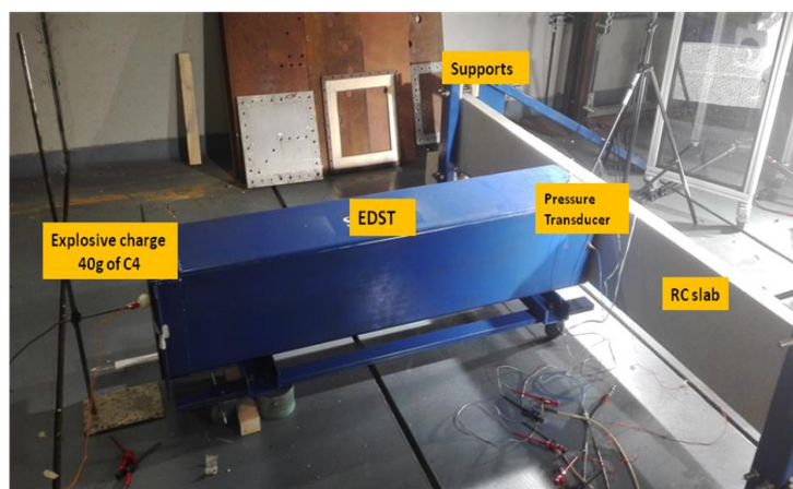
Figure 3. Experimental setup for blast tests
