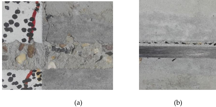
Figure 6. Debonding at the adhesive-concrete interface
