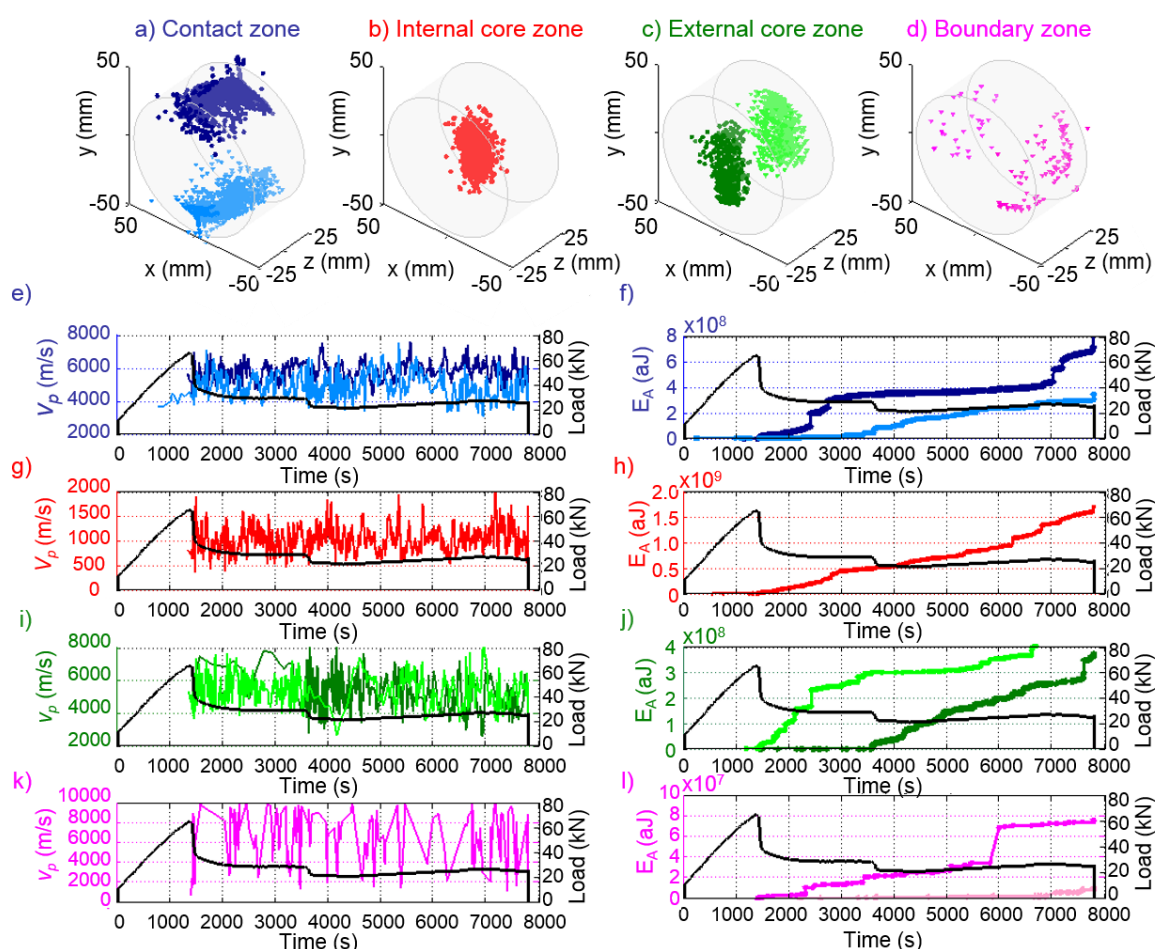
Figure 3. Distribution of damage obtained by application of CLAPW aVe to a monzogranite specimen under diametral compression test. Identified zones of damage (a to d) and distribution of v_p and E_A for contact zone (e and f), central core (g and h), external core (i and j) and boundary zone (k and l).
