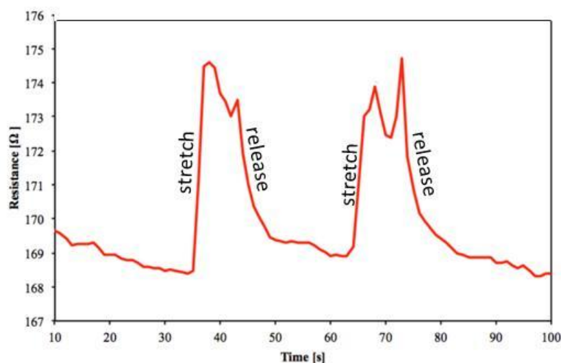
Figure 2: Electrical resistance changes when the nanocomposite is stretched.
