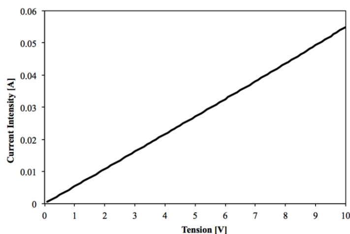
Figure 1: I/V test in stress-free condition.
