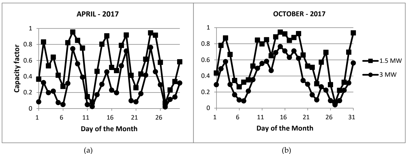
Figure 3. Daily variability of capacity factor for the two different types of wind turbines in Qollpana wind farm (a) April 2017; (b) October 2017.
