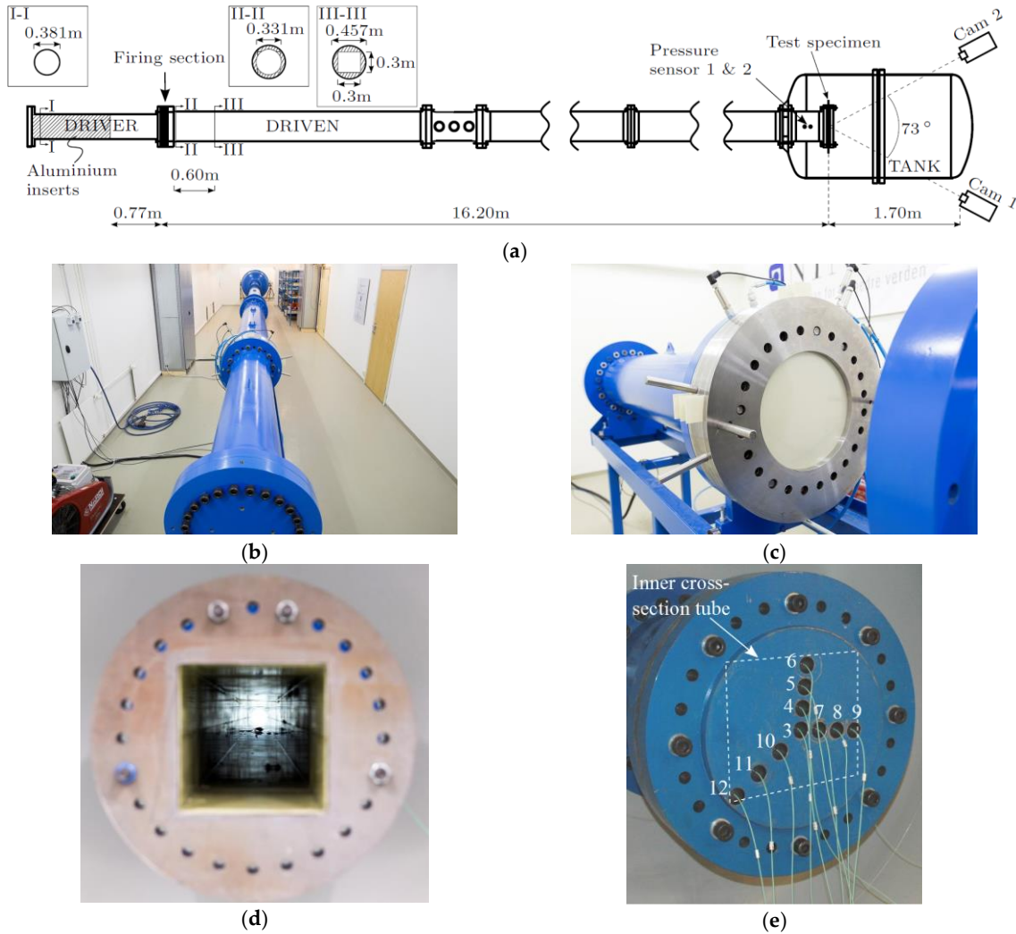
Figure 1. Experimental setup in the SIMLab Shock Tube Facility (SSTF) [5,9,10]: (a) Sketch of the experimental setup (seen from above); Picture of the (b) shock tube (seen from the driver section); (c) firing section (seen from the driven section); (d) internal cross-section driven section (seen from the tank); (e) massive steel plate (seen from the tank).
