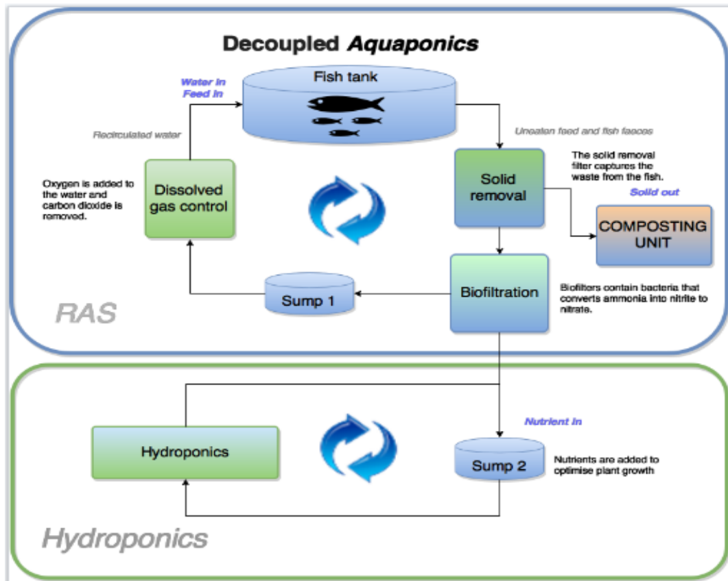
Figure 1. Schematic diagram of a decoupled aquaponic system [3]
