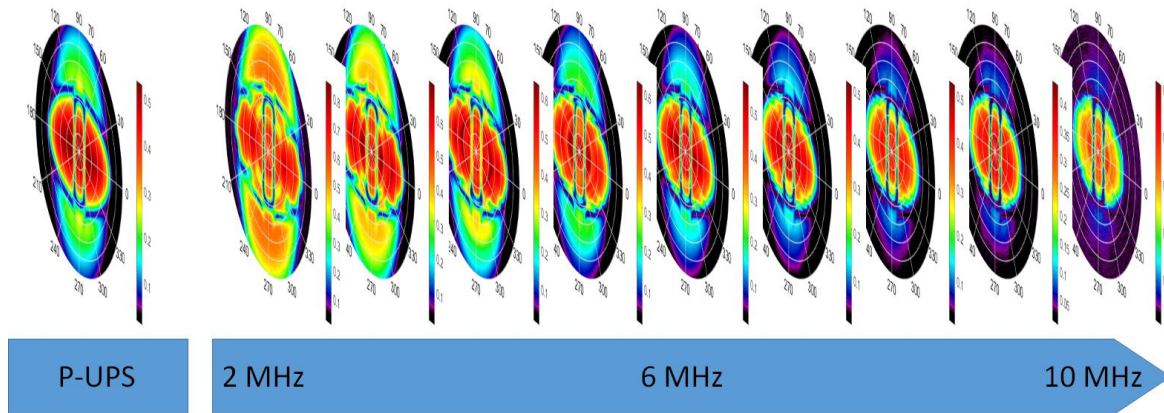
Figure 4. The typical amplitude polar diagram of the UPS technique for a [0°]8 carbon/epoxy composite (P-UPS) can be supplemented with a spectroscopic analysis to provide a large number of S-UPS diagrams for different frequency bands.
