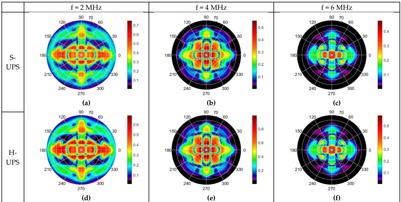
Figure 7. (a)(b)(c) Polar scan images of a [0 2 ,90 2 ]S carbon/epoxy composite obtained by the S-UPS for frequencies of 2 MHz, 4 MHz and 6 MHz respectively compared to (d)(e)(f) polar scan images obtained for separate H-UPS measurements of the same sample and for the same respective frequencies.
