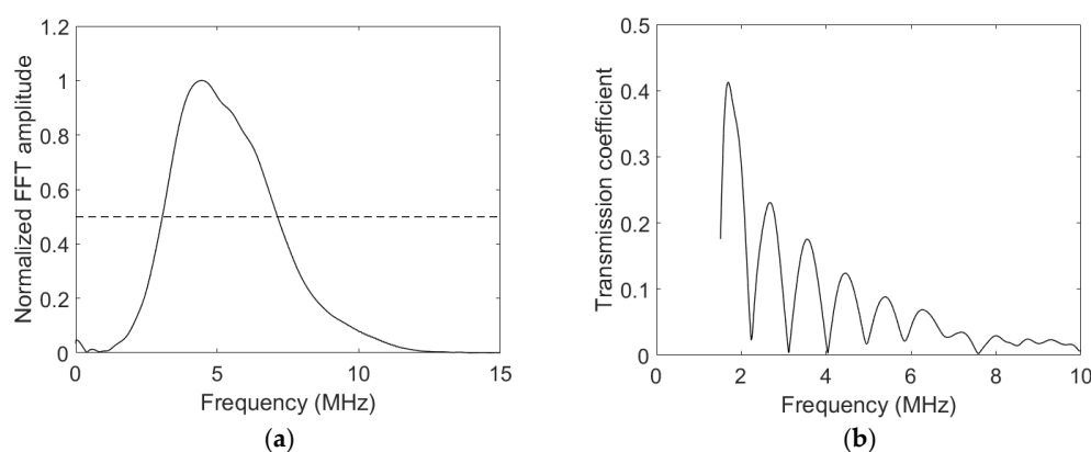
Figure 3. (a) Frequency amplitude spectrum of the transducers used in the experiment for the water reference. (b) Example of the transmission coefficient spectrum for a UD composite at \theta = 35^\circ , \varphi = 60^\circ .
