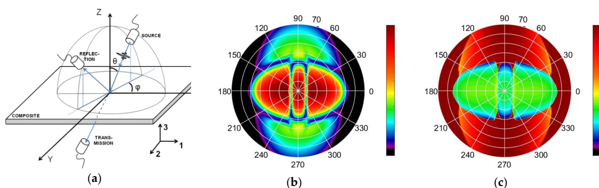
Figure 1. (a) Principle of the Pulsed Ultrasonic Polar Scan technique (P-UPS). Experimental P-UPS recording for a [0^\circ]_8 carbon/epoxy composite: (b) amplitude and (c) TOF.
