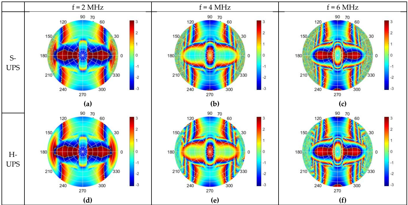
Figure 6. (a)(b)(c) Phase diagrams of a [0]8 carbon/epoxy composite obtained by the S-UPS for frequencies of 2 MHz, 4 MHz and 6 MHz respectively compared to (d)(e)(f) images obtained for H-UPS measurements for the same respective frequencies.
