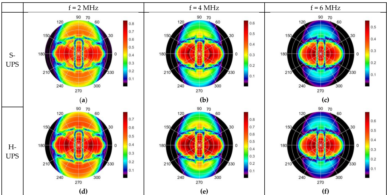
Figure 5. (a)(b)(c) S-UPS images of a [0]8 carbon/epoxy composite for frequencies of 2 MHz, 4 MHz and 6 MHz respectively compared to (d)(e)(f) polar scan images obtained for separate H-UPS measurements of the same sample and for the same respective frequencies.
