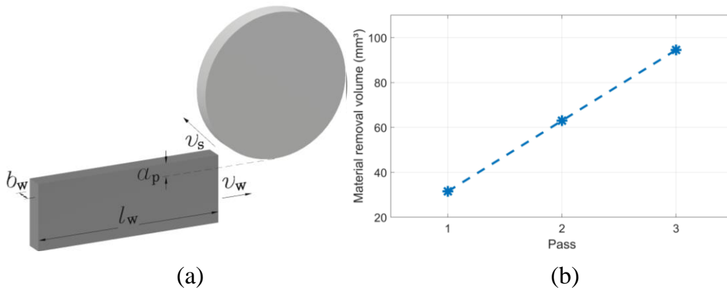
Figure 1. (a) Schematic for grinding process with cutting parameters b) material removal volume as function of grinding pass
