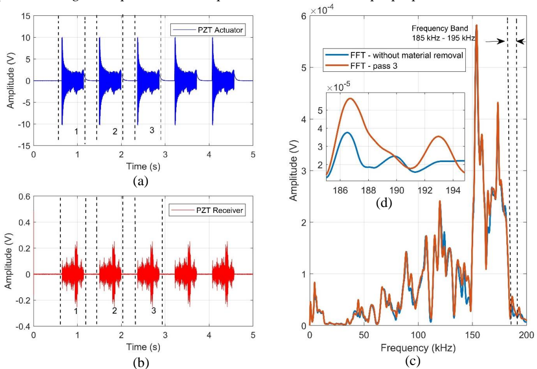
Figure 2. Emitted signal (a) and received signals (b); spectrum for two workpiece conditions, (c) spectrum magnification 186 – 194 kHz (d)
