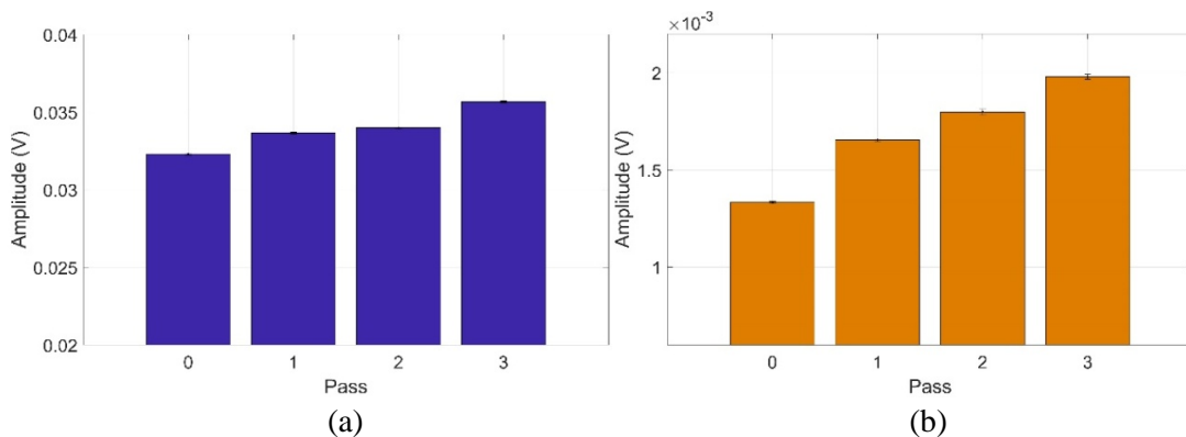
Figure 3. Mean RMS and standard deviation – raw signals (a) and filtered signals (b)
